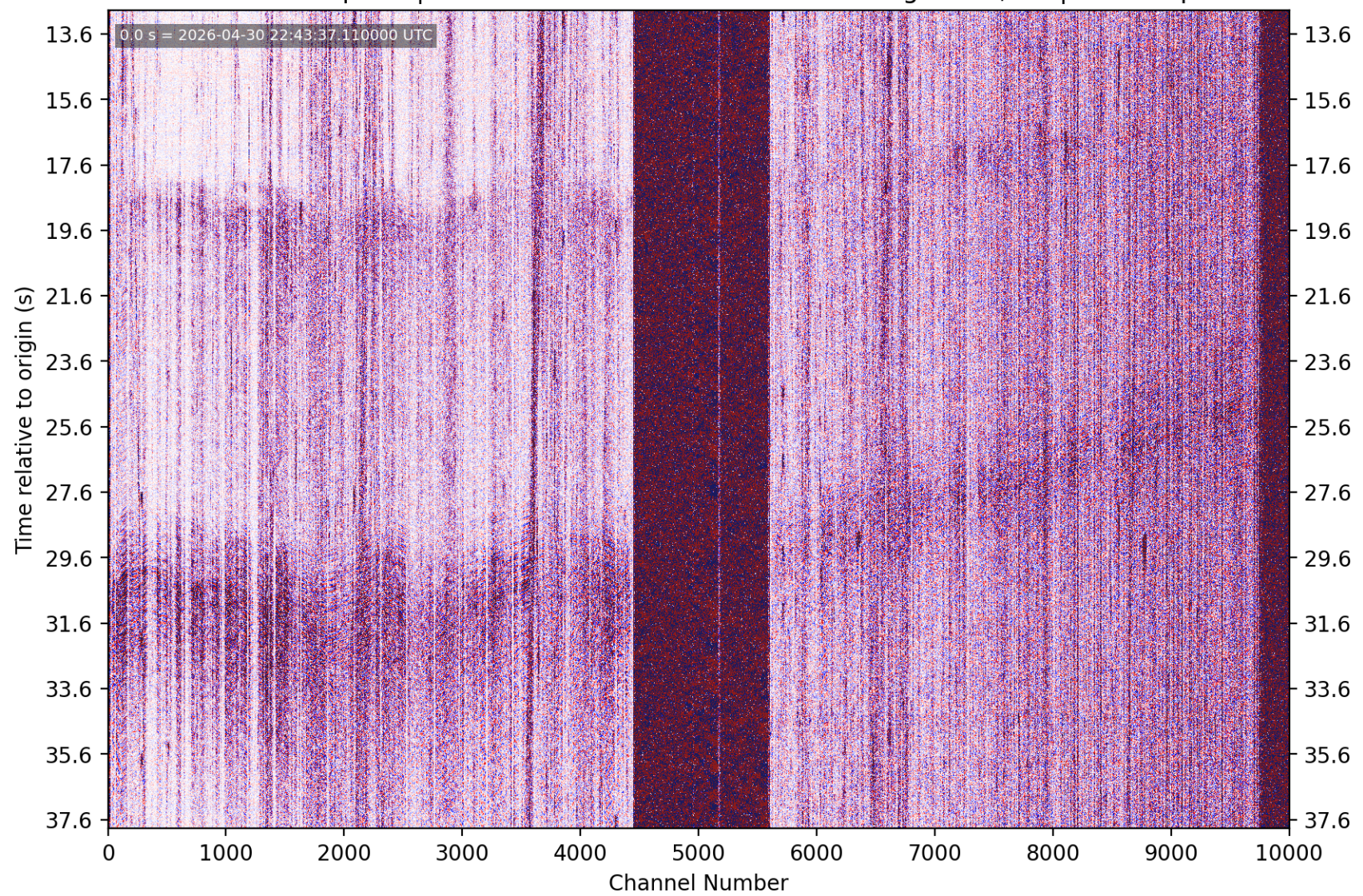
PhaseNet-DAS picks | nc75354597 M2.77 14 km N of Morgan Hill, CA | without picks
