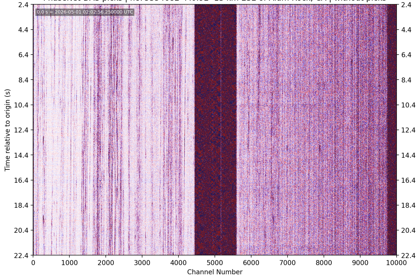
PhaseNet-DAS picks | nc75354682 M0.92 13 km ESE of Alum Rock, CA | without picks
