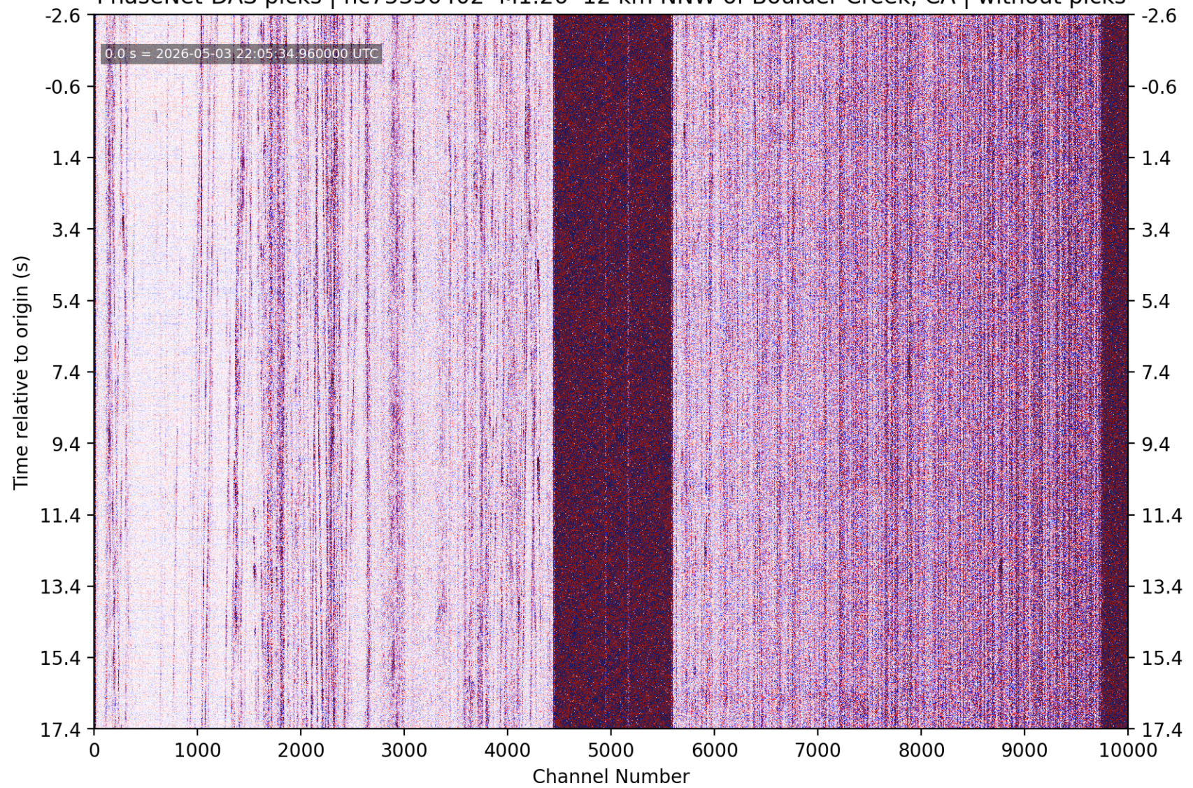
PhaseNet-DAS picks | nc75356402 M1.26 12 km NNW of Boulder Creek, CA | without picks
