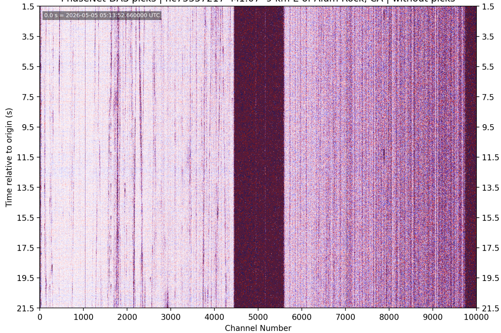
PhaseNet-DAS picks | nc75357217 M1.07 9 km E of Alum Rock, CA | without picks
