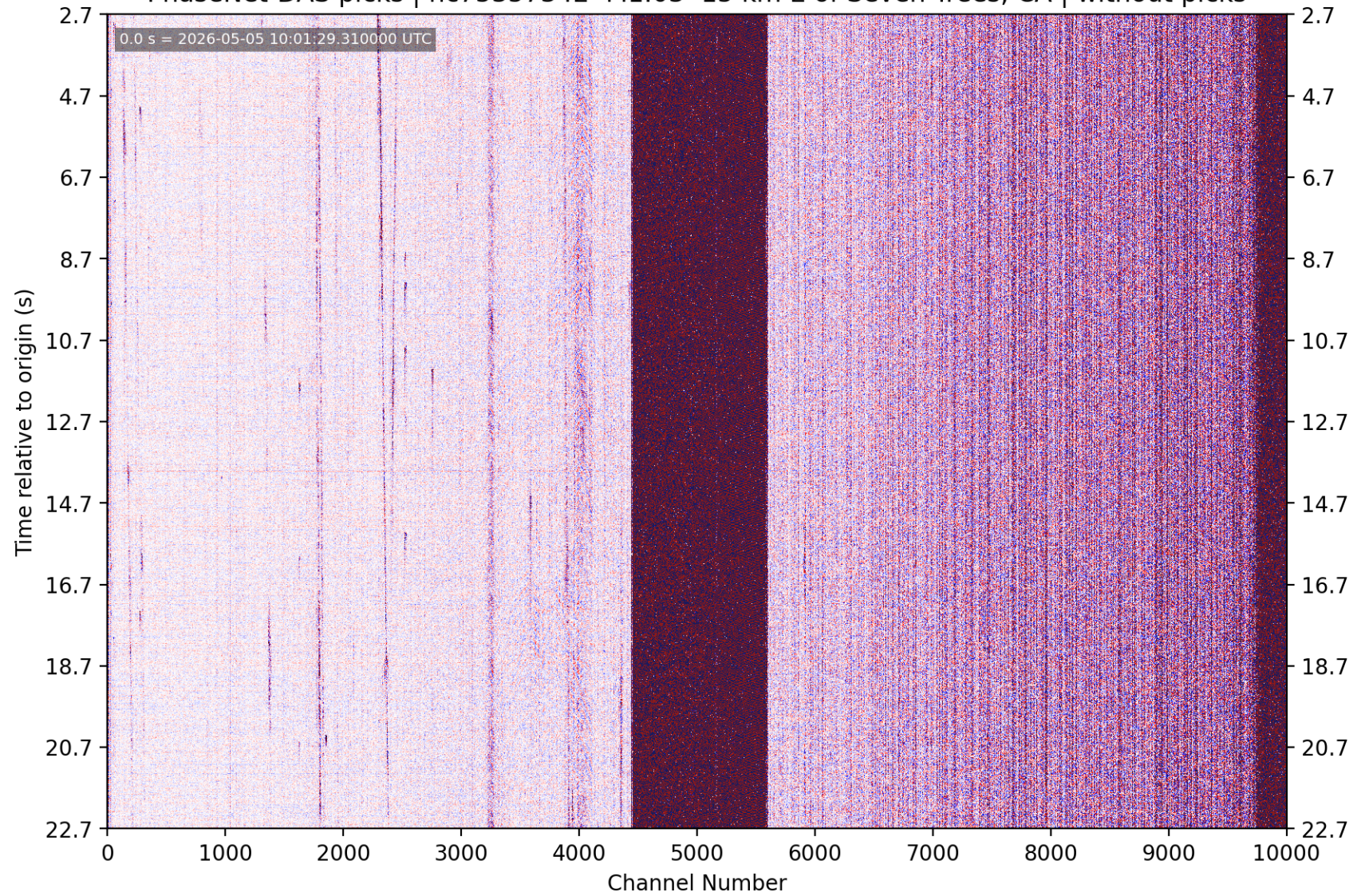
PhaseNet-DAS picks | nc75357342 M1.03 15 km E of Seven Trees, CA | without picks
