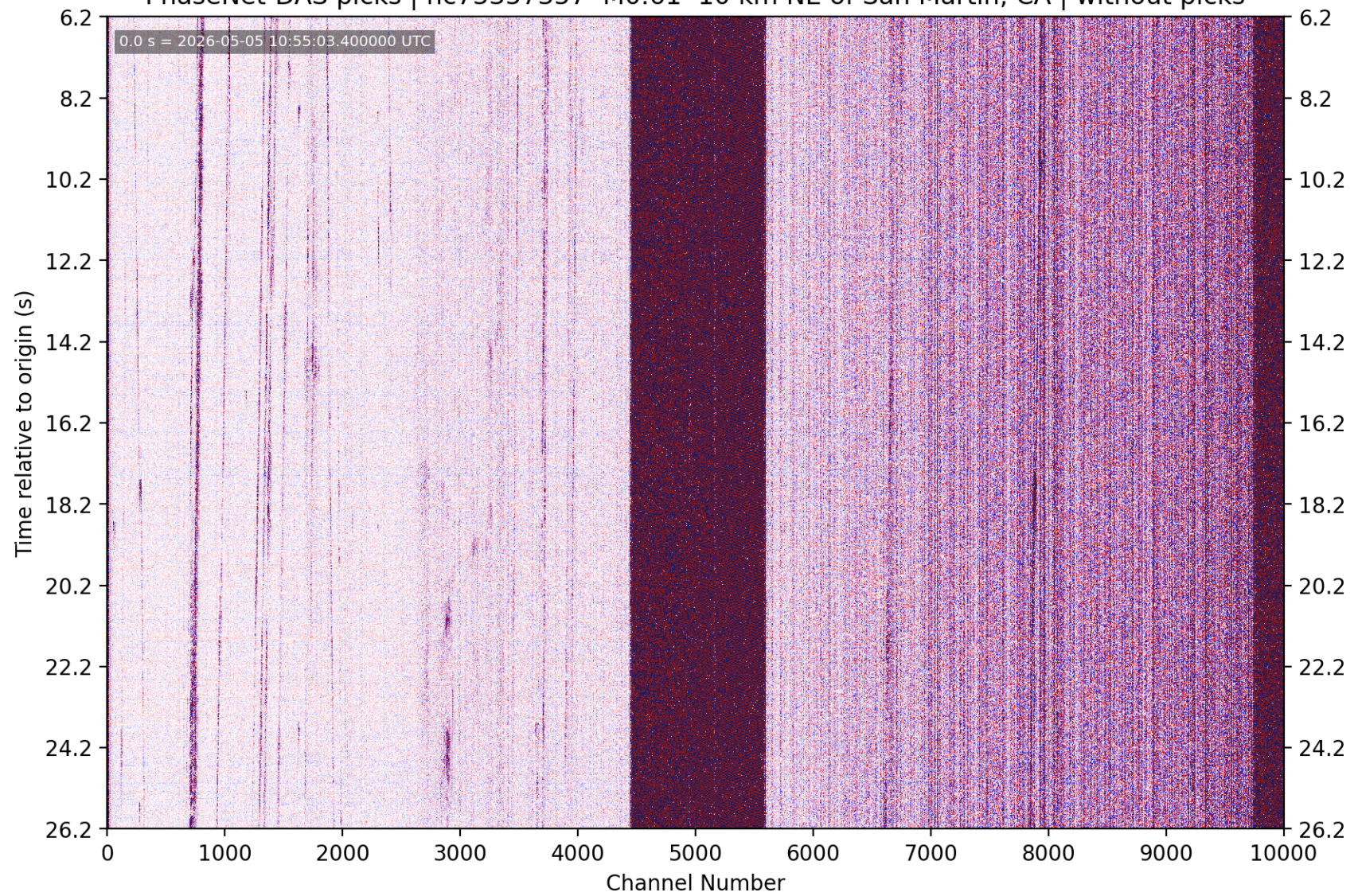
PhaseNet-DAS picks | nc75357357 M0.61 10 km NE of San Martin, CA | without picks
