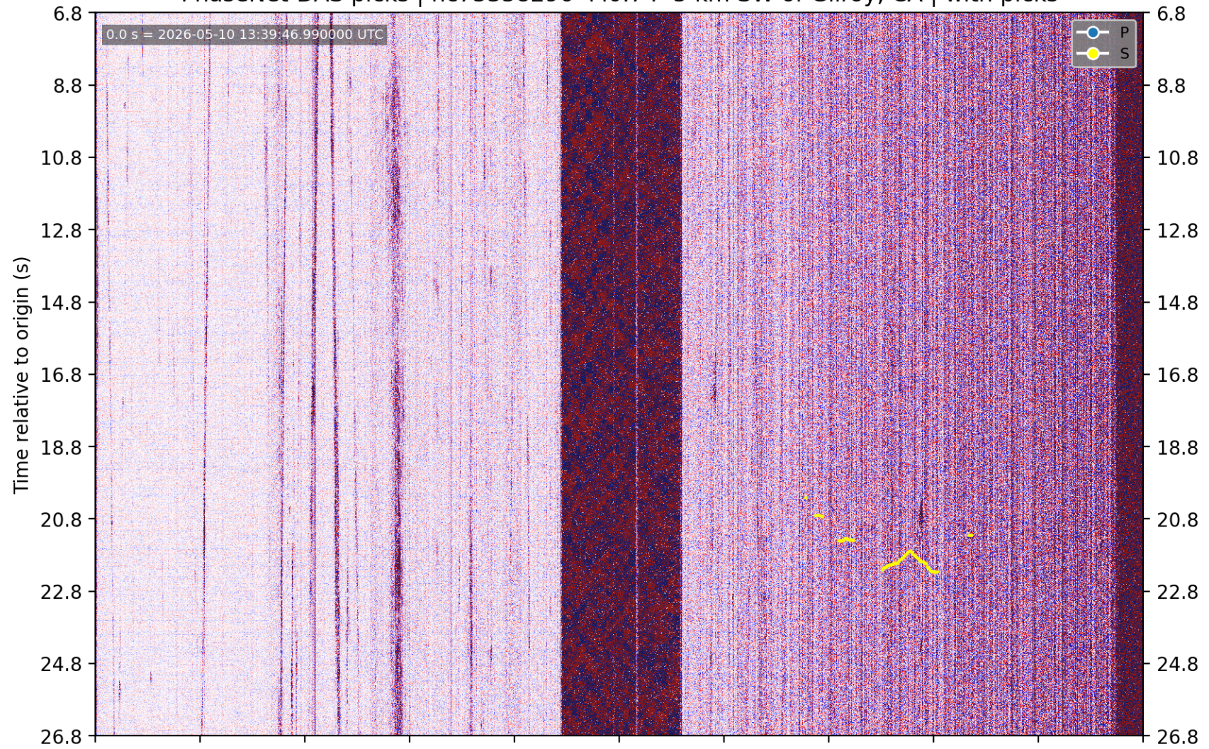
PhaseNet-DAS picks | nc75358296 M0.74 5 km SW of Gilroy, CA | without picks
