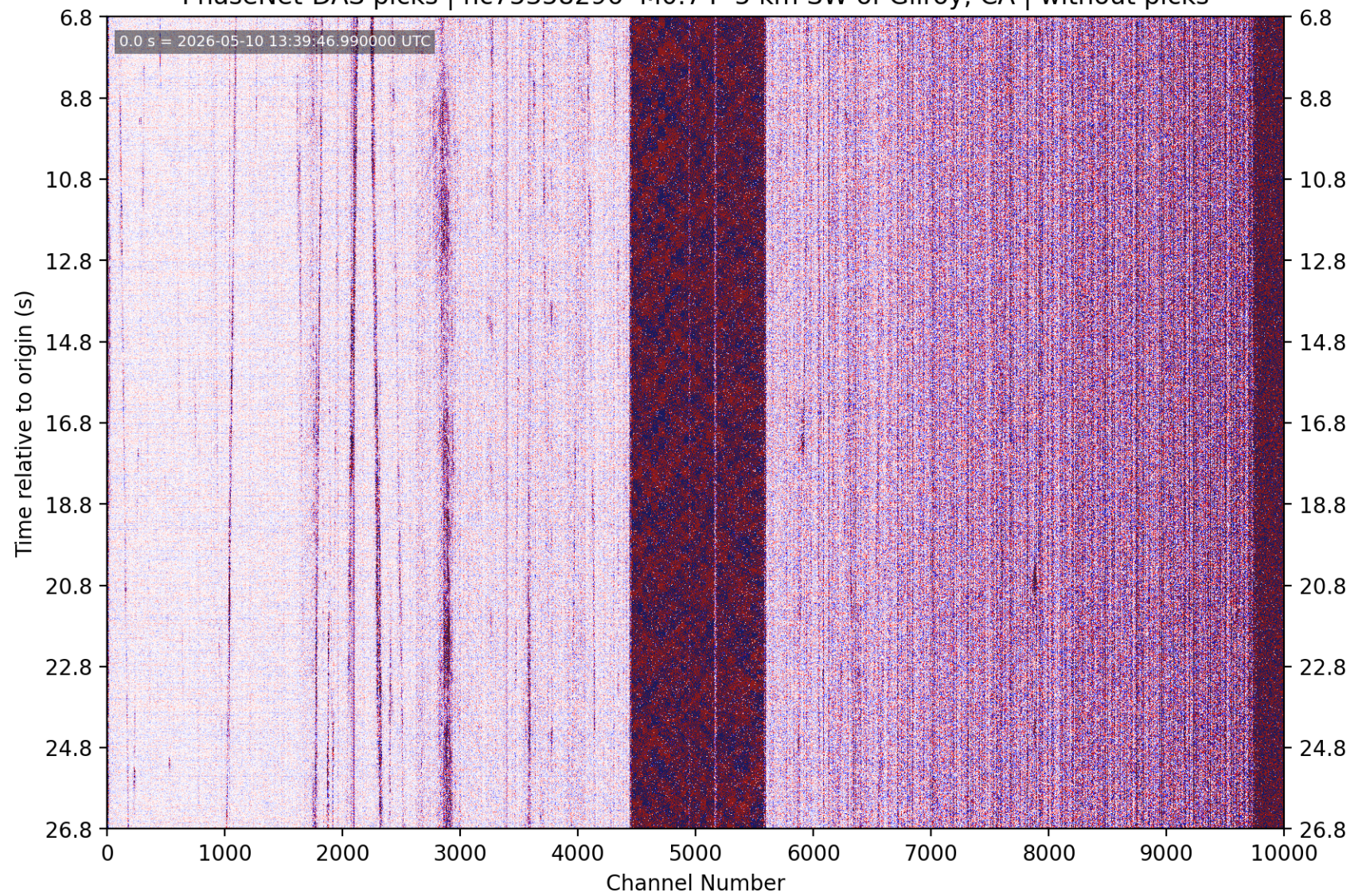
PhaseNet-DAS picks | nc75358296 M0.74 5 km SW of Gilroy, CA | without picks
