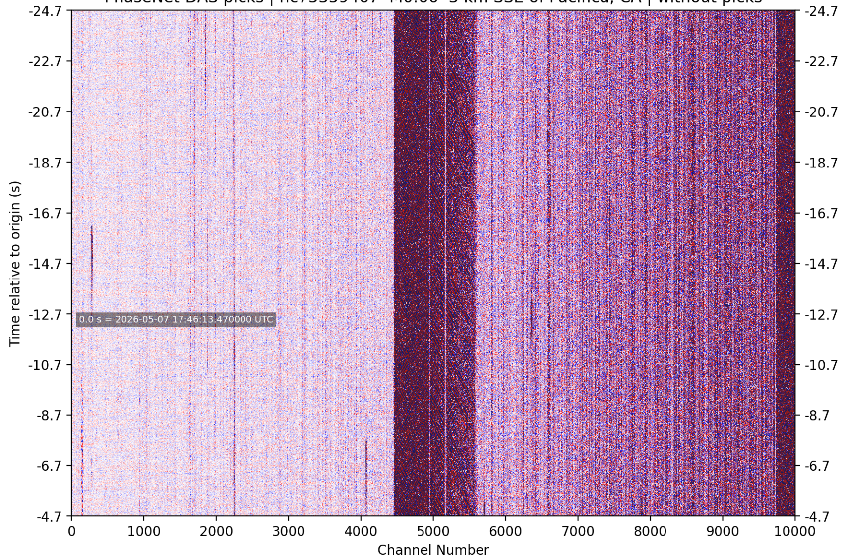
PhaseNet-DAS picks | nc75359467 M0.66 3 km SSE of Pacifica, CA | without picks
