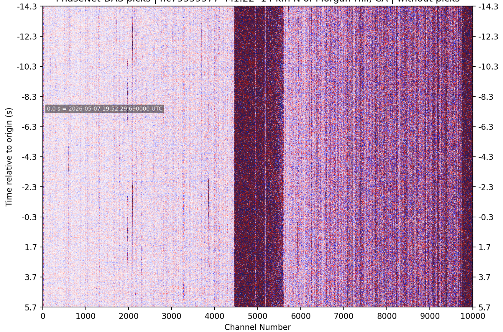
PhaseNet-DAS picks | nc75359577 M1.22 14 km N of Morgan Hill, CA | without picks
