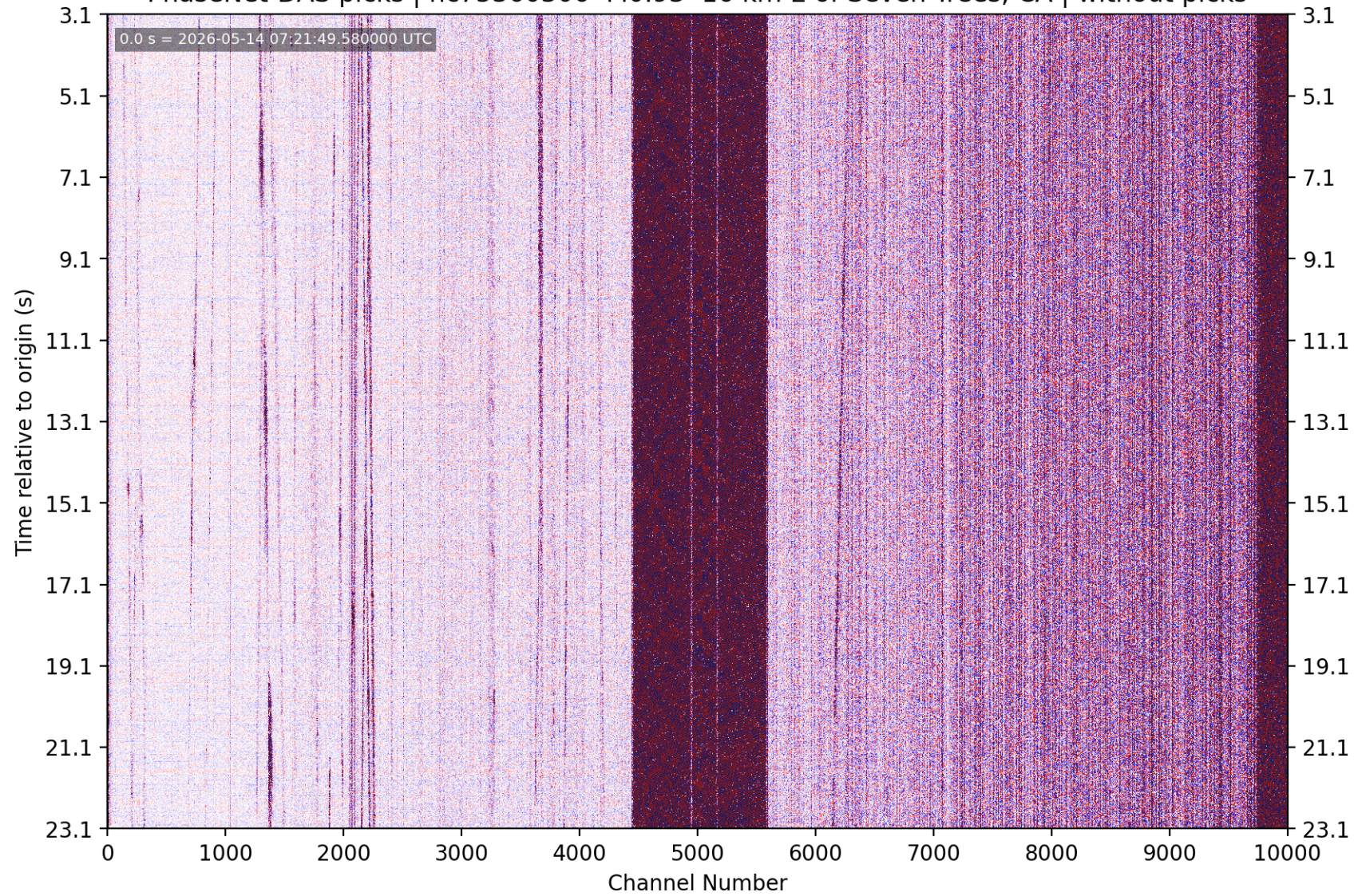
PhaseNet-DAS picks | nc75360306 M0.93 16 km E of Seven Trees, CA | without picks
