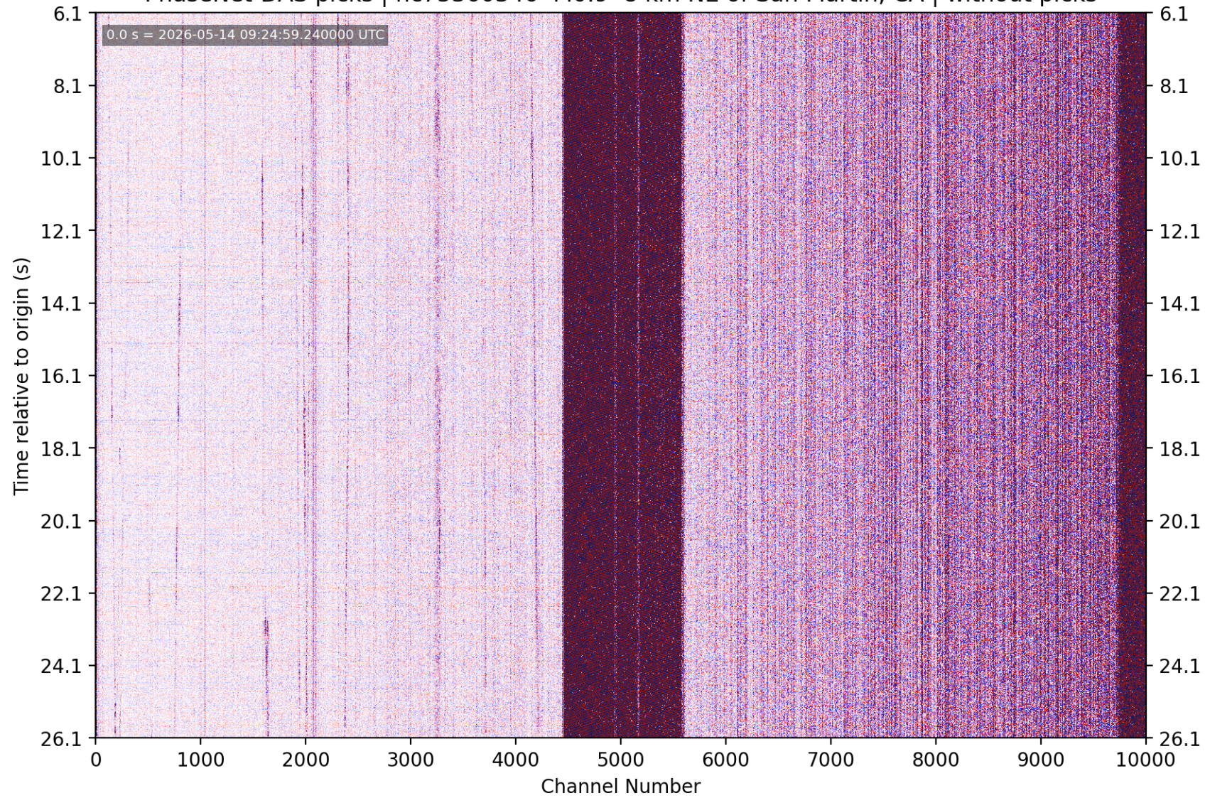
PhaseNet-DAS picks | nc75360346 M0.9 8 km NE of San Martin, CA | without picks
