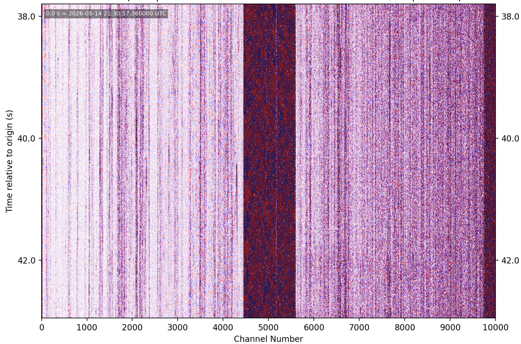
PhaseNet-DAS picks | nc75360561 M0.91 15 km ENE of Alum Rock, CA | without picks
