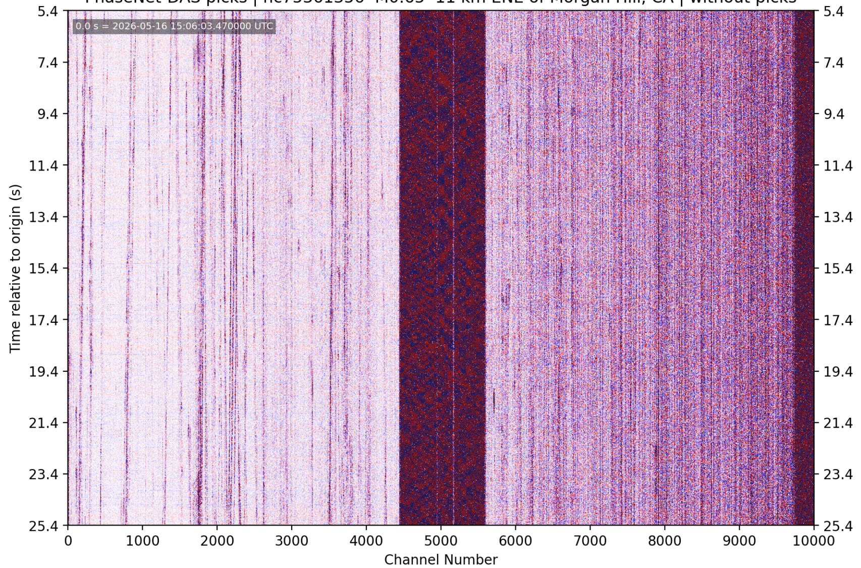
PhaseNet-DAS picks | nc75361356 M0.65 11 km ENE of Morgan Hill, CA | without picks
