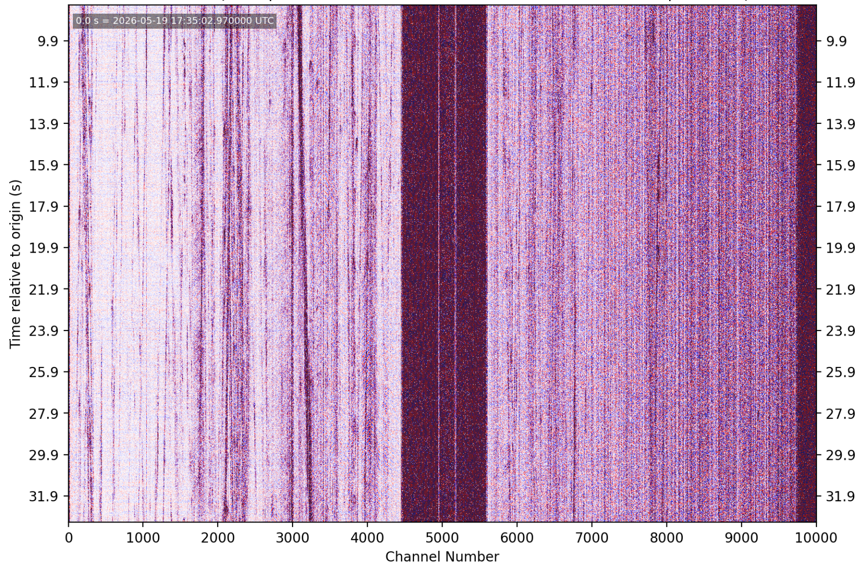
PhaseNet-DAS picks | nc75365717 M1.45 11 km E of Alum Rock, CA | without picks
