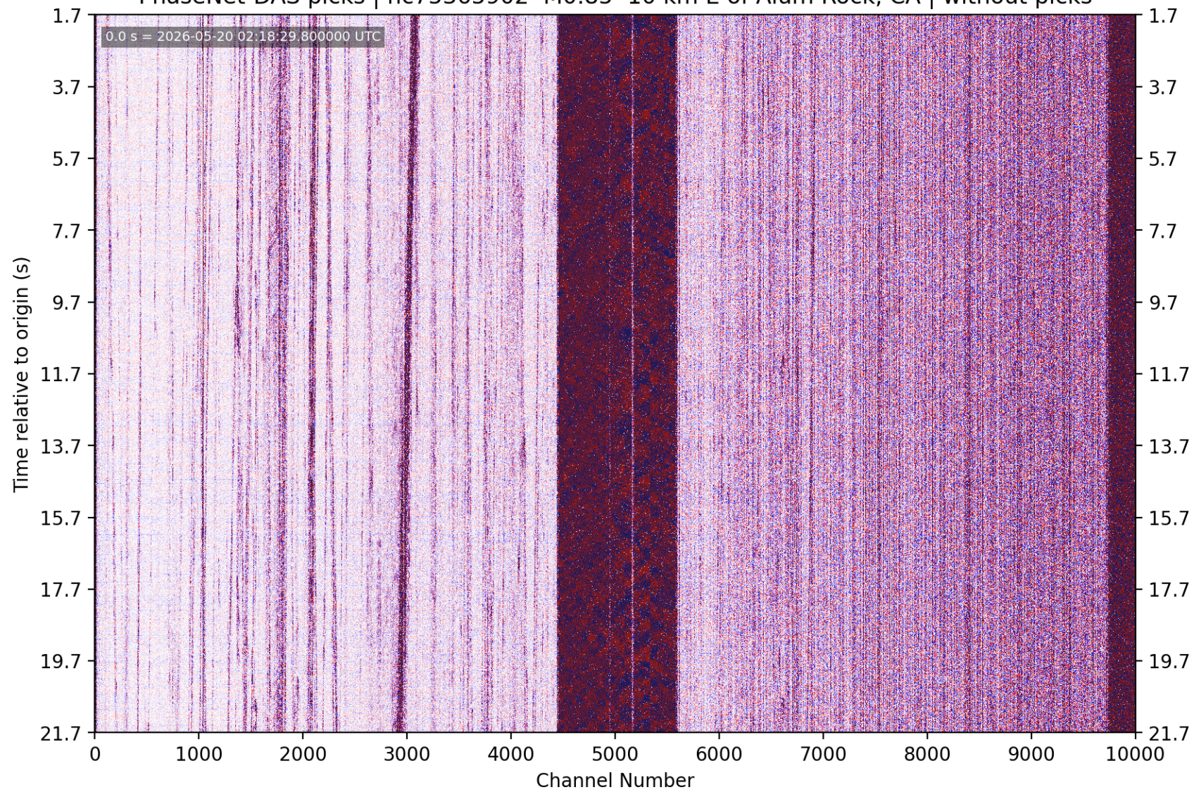
PhaseNet-DAS picks | nc75365902 M0.85 10 km E of Alum Rock, CA | without picks
