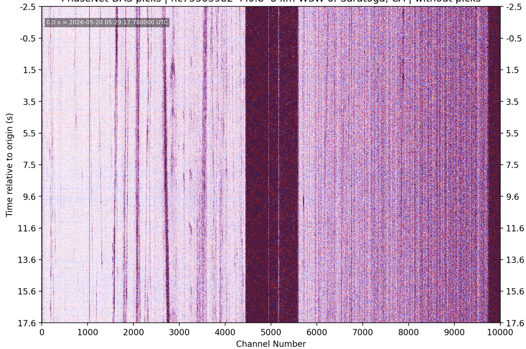
PhaseNet-DAS picks | nc75365982 M0.8 8 km WSW of Saratoga, CA | without picks
