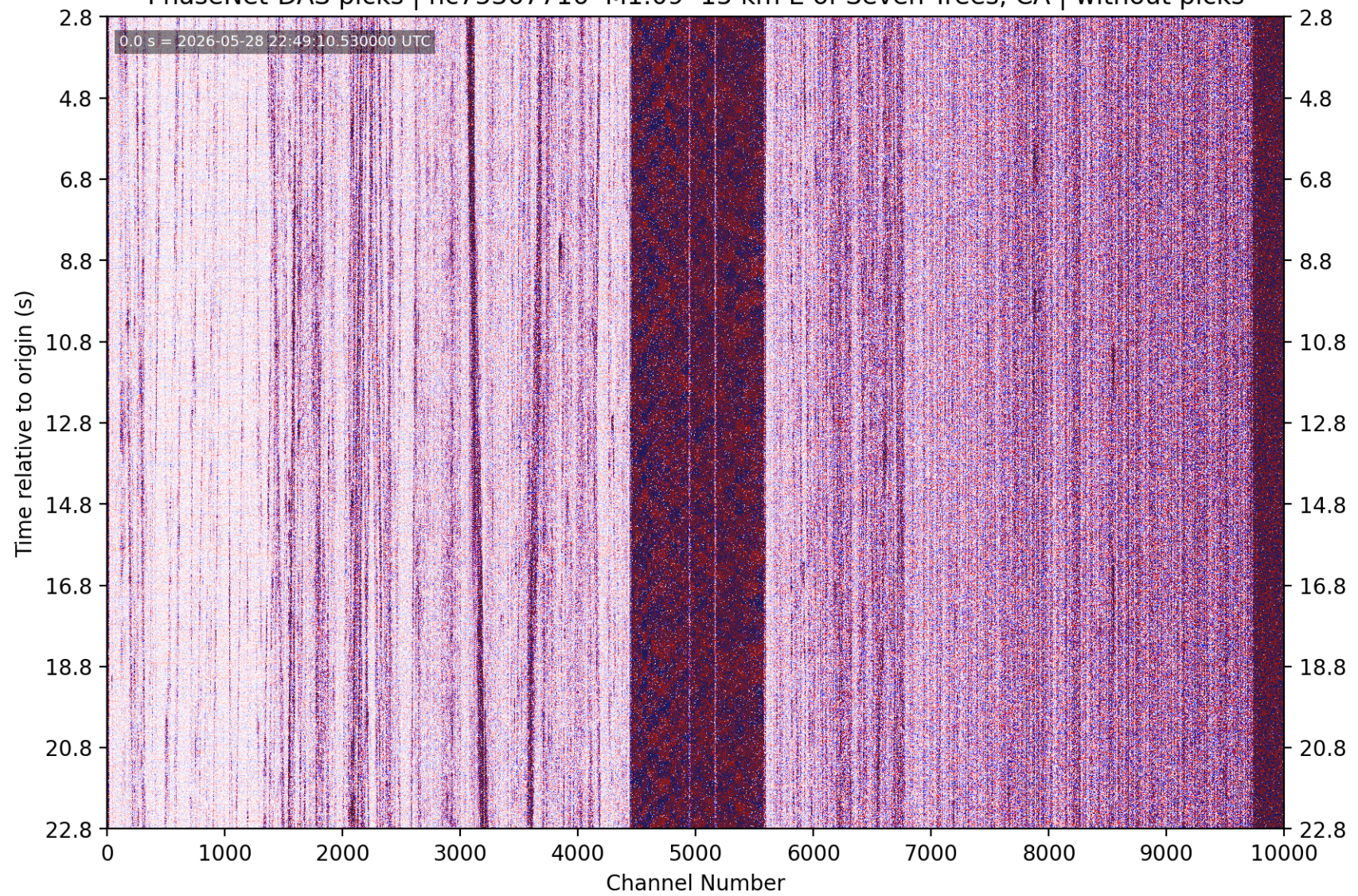
PhaseNet-DAS picks | nc75367716 M1.09 15 km E of Seven Trees, CA | without picks
