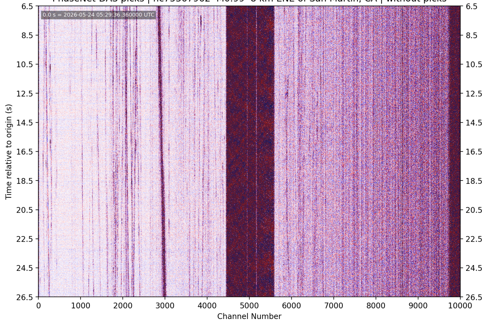
PhaseNet-DAS picks | nc75367962 M0.99 8 km ENE of San Martin, CA | without picks
