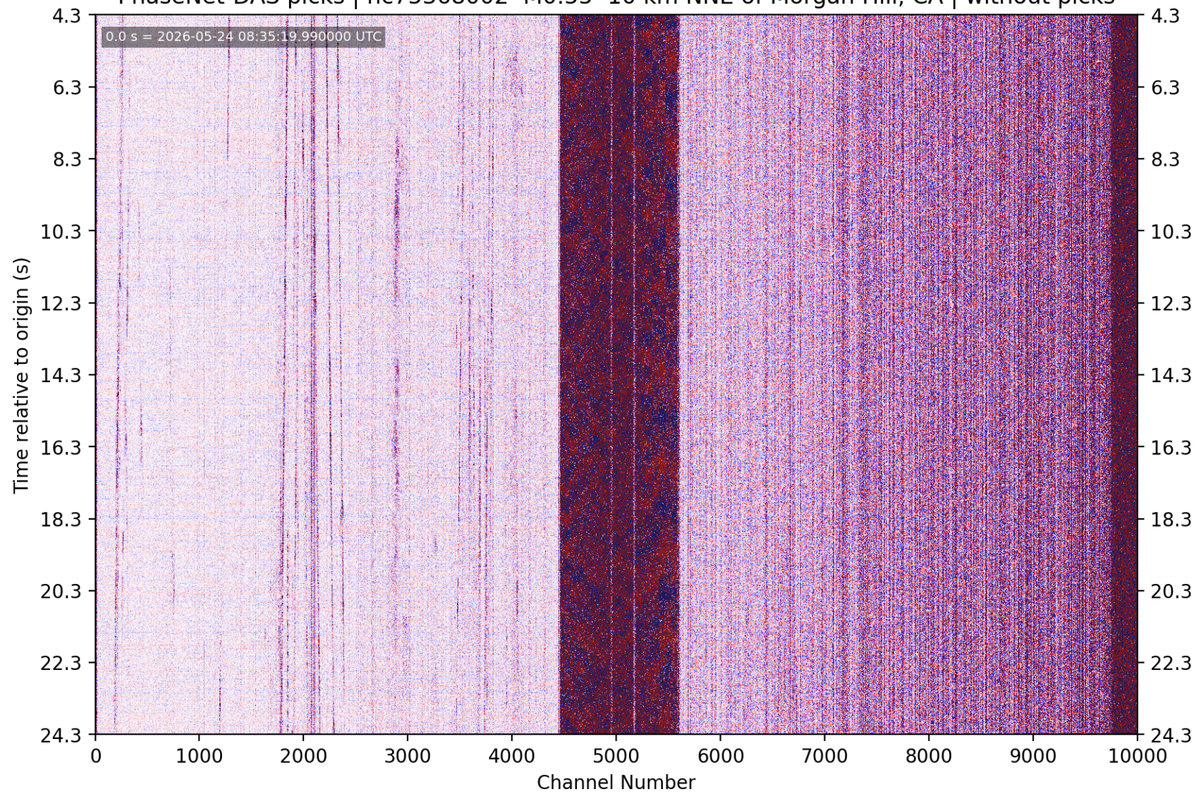
PhaseNet-DAS picks | nc75368002 M0.55 10 km NNE of Morgan Hill, CA | without picks
