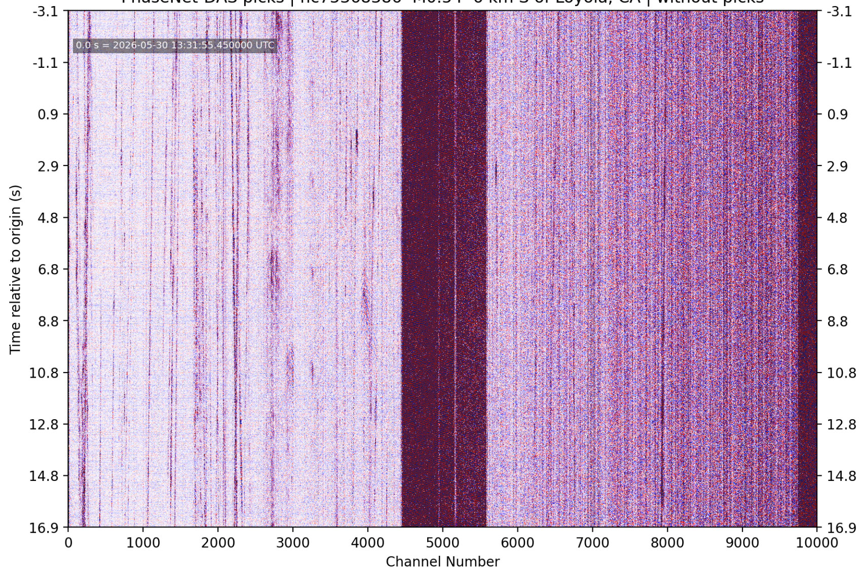
PhaseNet-DAS picks | nc75368386 M0.54 6 km S of Loyola, CA | without picks
