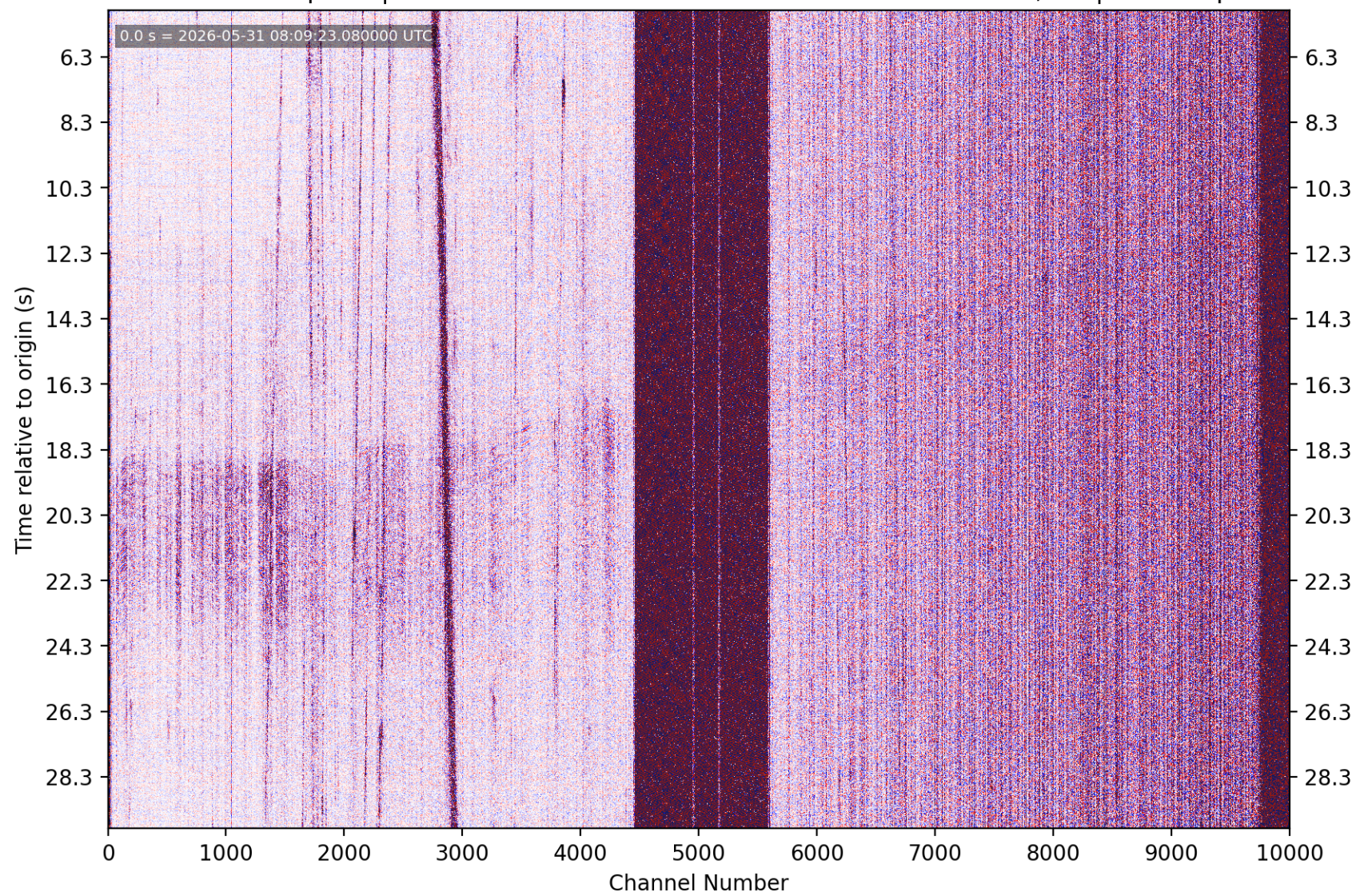
PhaseNet-DAS picks | nc75368636 M2.4 21 km WNW of Boulder Creek, CA | without picks
