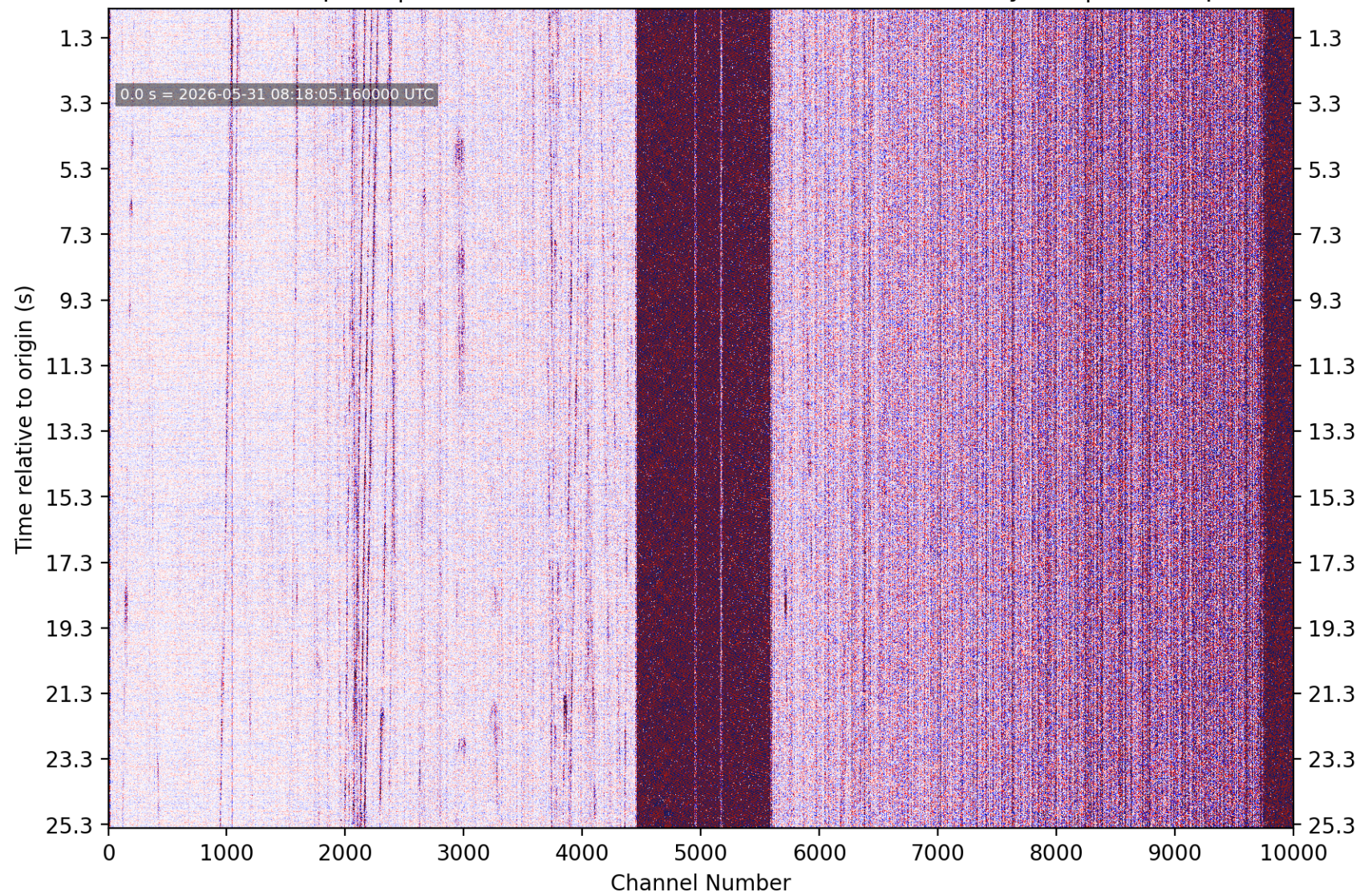
PhaseNet-DAS picks | nc75368651 M1.47 6 km SSE of Portola Valley, CA | without picks
