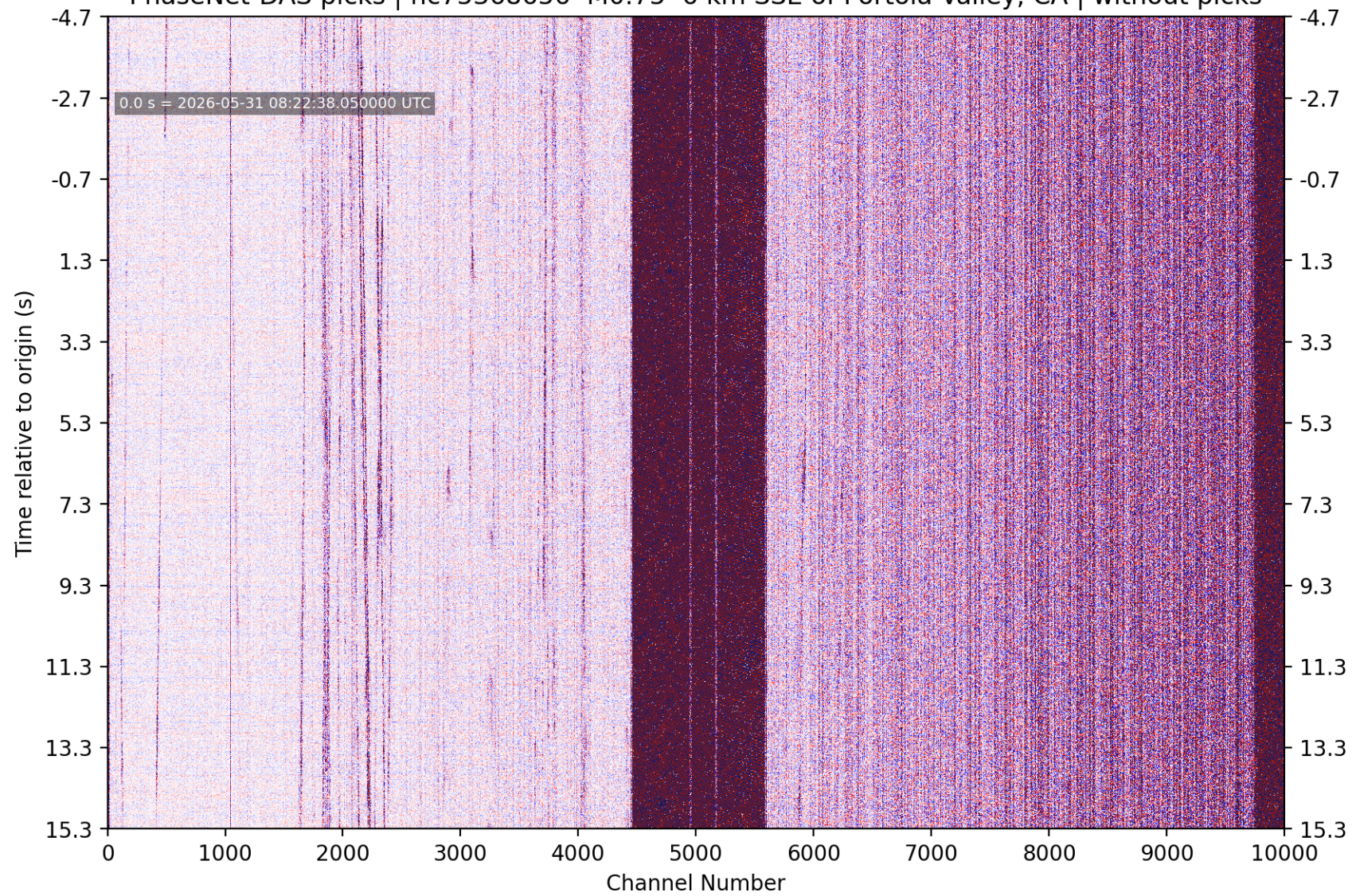
PhaseNet-DAS picks | nc75368656 M0.75 6 km SSE of Portola Valley, CA | without picks
