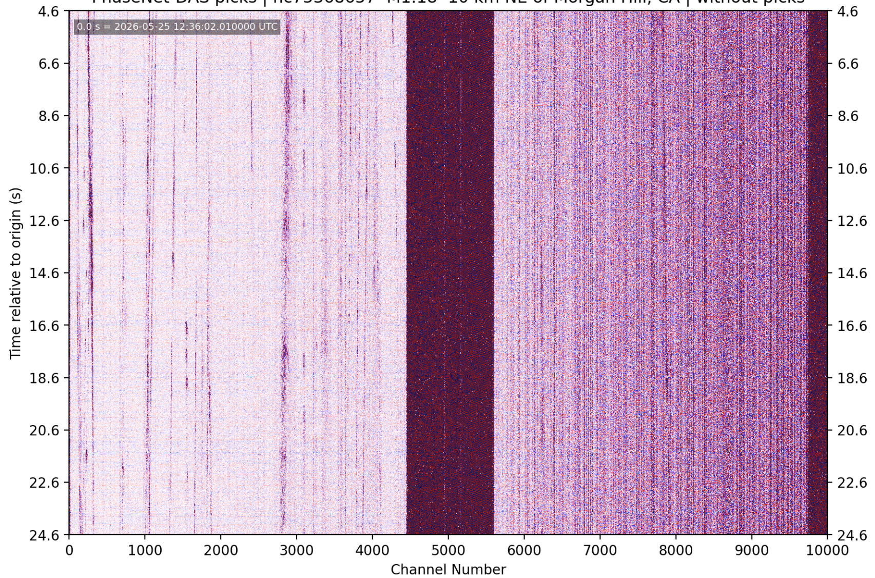
PhaseNet-DAS picks | nc75368657 M1.18 10 km NE of Morgan Hill, CA | without picks
