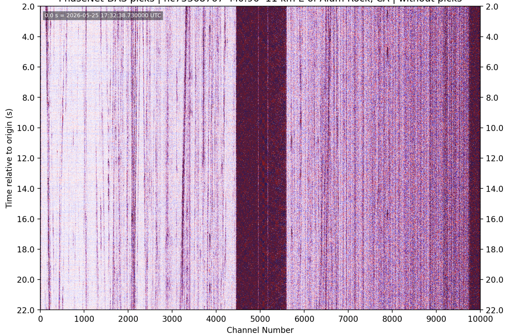
PhaseNet-DAS picks | nc75368767 M0.96 11 km E of Alum Rock, CA | without picks
