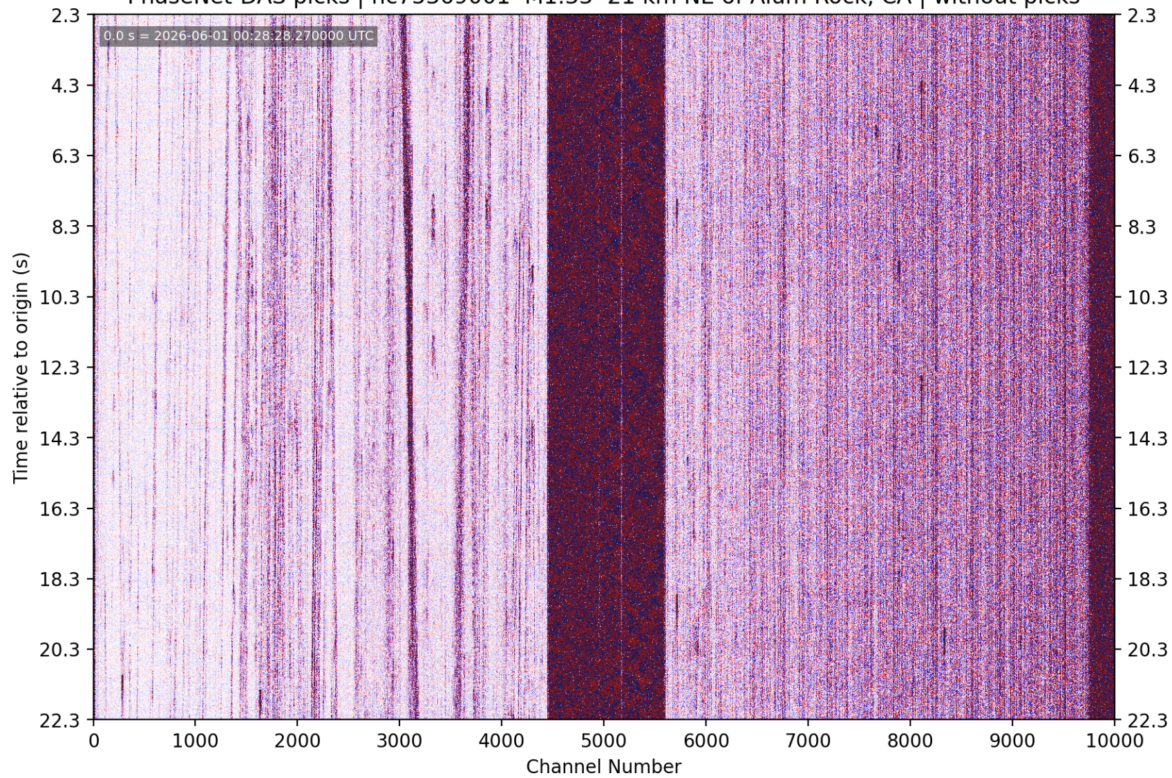
PhaseNet-DAS picks | nc75369001 M1.33 21 km NE of Alum Rock, CA | without picks
