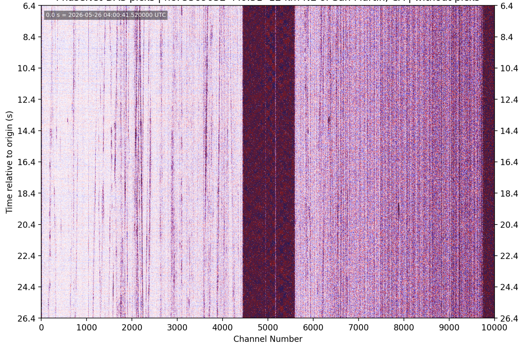
PhaseNet-DAS picks | nc75369032 M0.31 12 km NE of San Martin, CA | without picks
