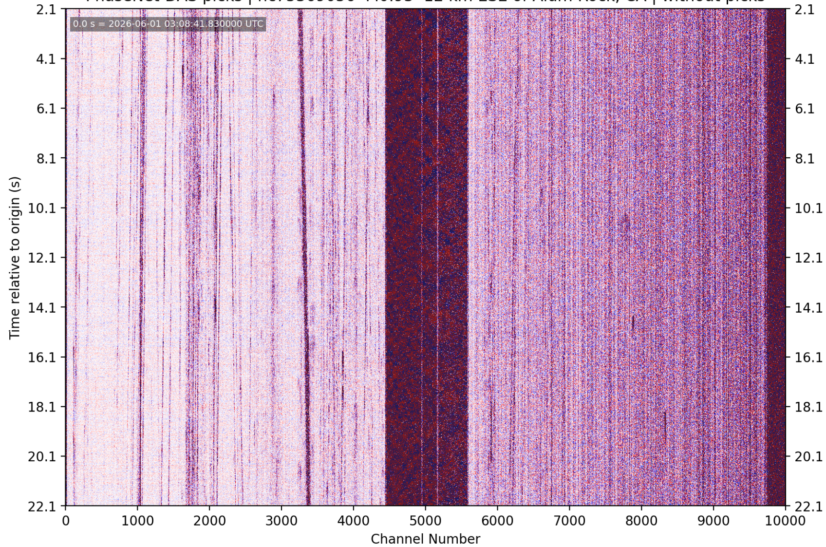
PhaseNet-DAS picks | nc75369056 M0.93 12 km ESE of Alum Rock, CA | without picks
