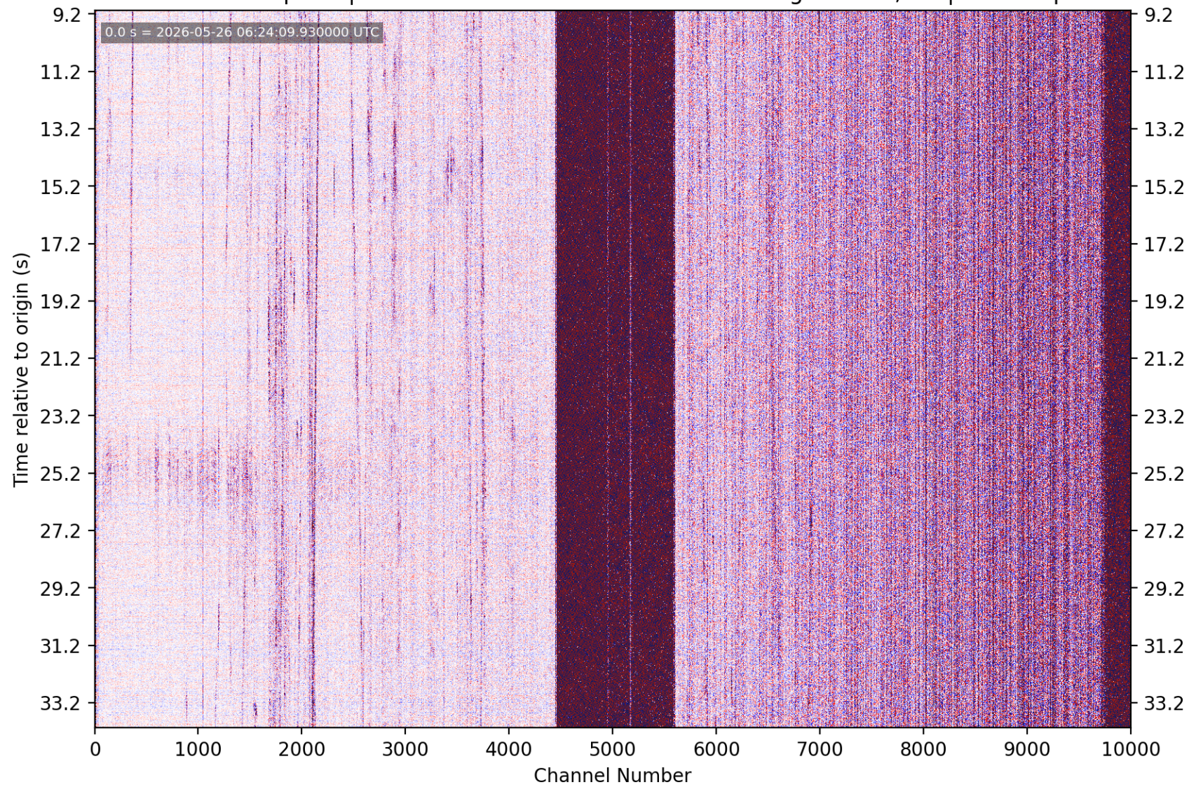
PhaseNet-DAS picks | nc75369082 M1.97 6 km SE of Lexington Hills, CA | without picks
