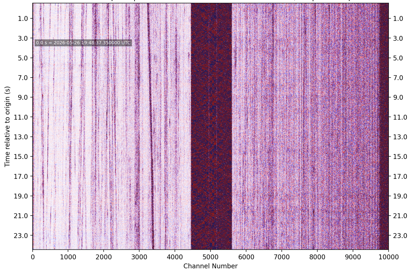
PhaseNet-DAS picks | nc75369377 M0.78 5 km SE of Pacifica, CA | without picks
