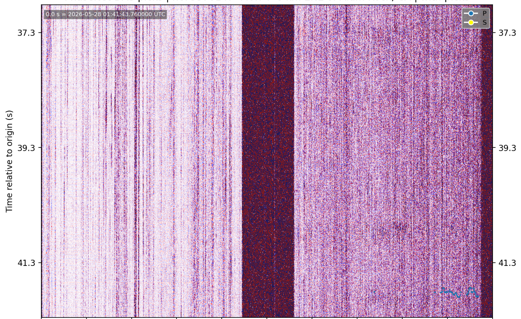
PhaseNet-DAS picks | nc75370147 M0.74 8 km ENE of Alum Rock, CA | without picks
