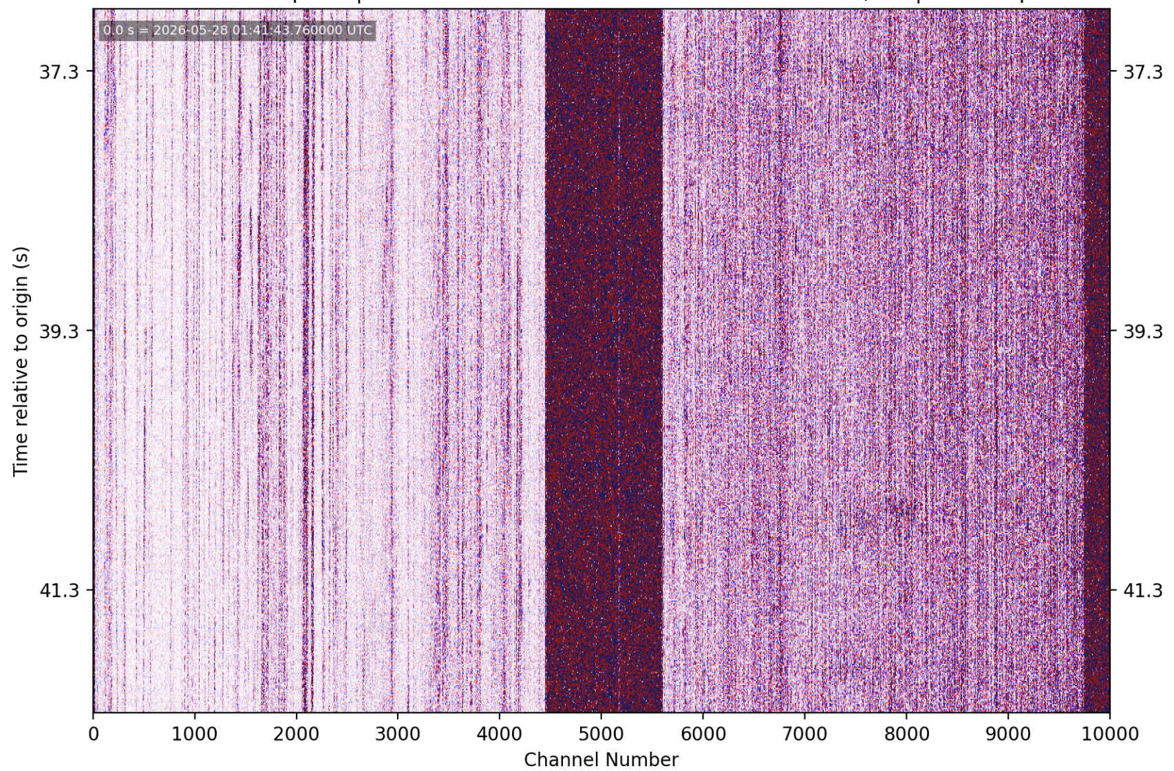
PhaseNet-DAS picks | nc75370147 M0.74 8 km ENE of Alum Rock, CA | without picks
