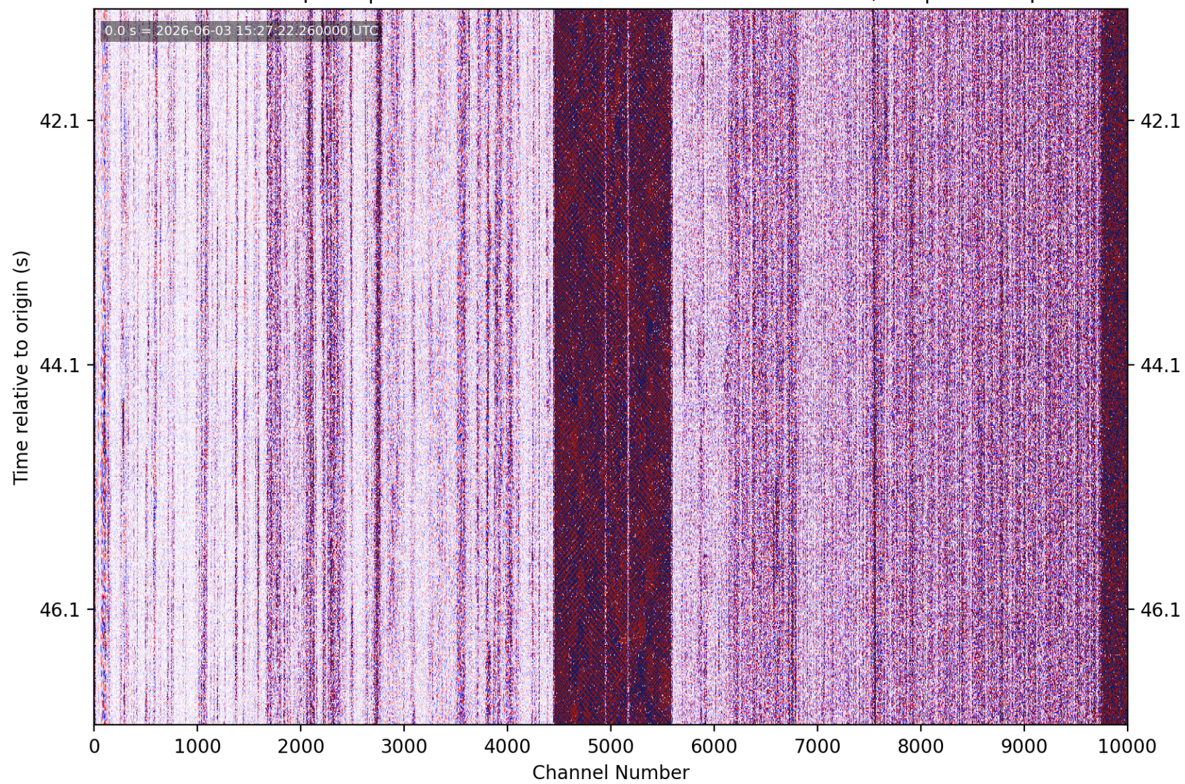
PhaseNet-DAS picks | nc75370251 M0.83 9 km NE of San Martin, CA | without picks
