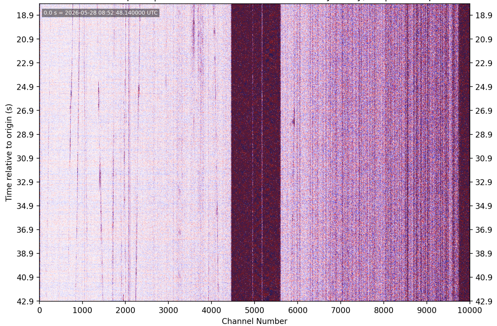
PhaseNet-DAS picks | nc75370292 M0.9 10 km NE of Day Valley, CA | without picks
