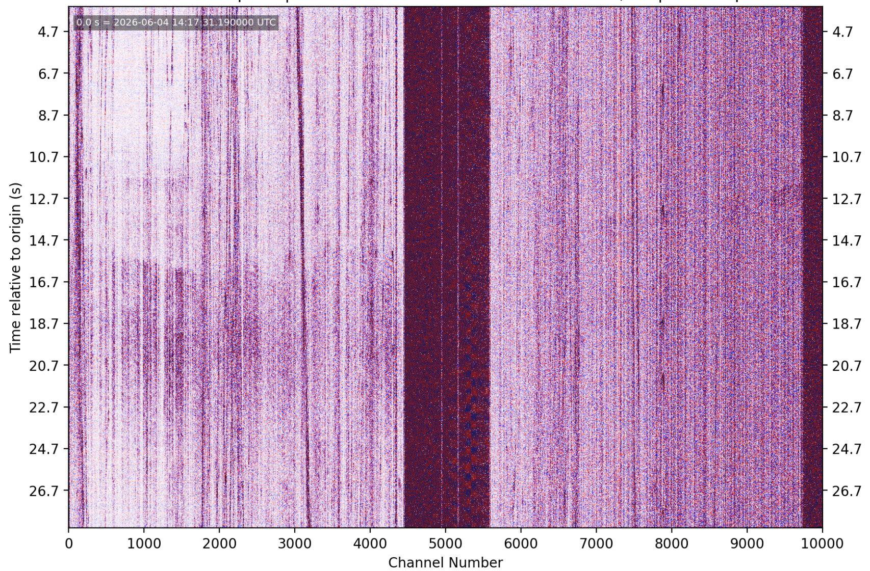
PhaseNet-DAS picks | nc75370736 M2.65 7 km E of Fremont, CA | without picks
