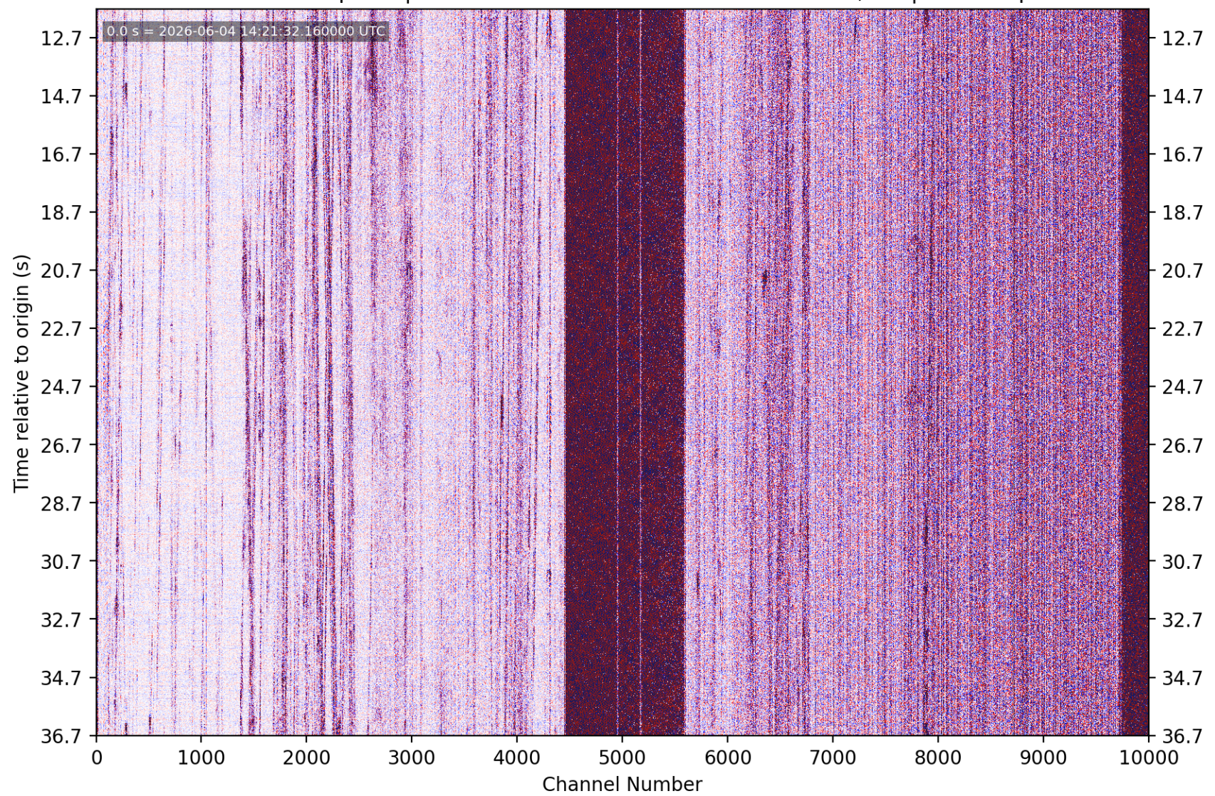
PhaseNet-DAS picks | nc75370746 M1.0 7 km E of Fremont, CA | without picks
