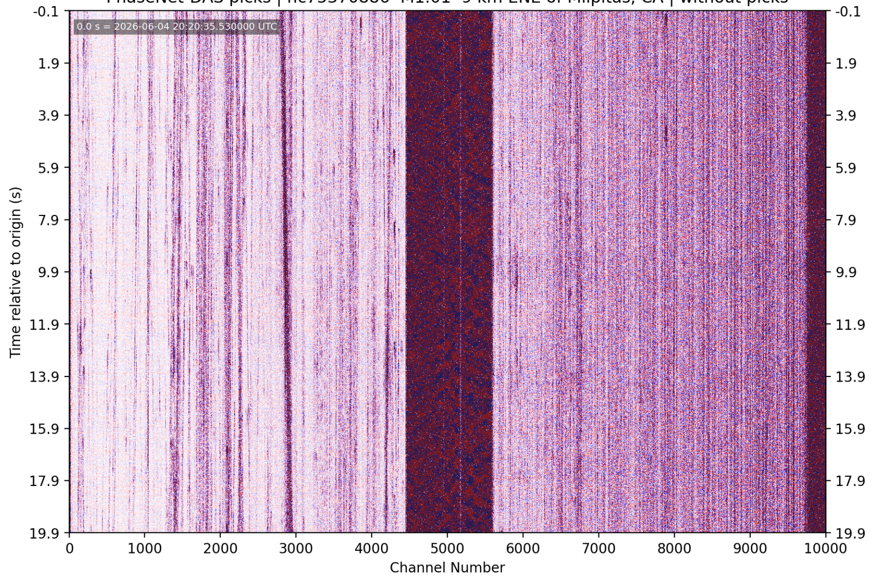
PhaseNet-DAS picks | nc75370886 M1.01 9 km ENE of Milpitas, CA | without picks
