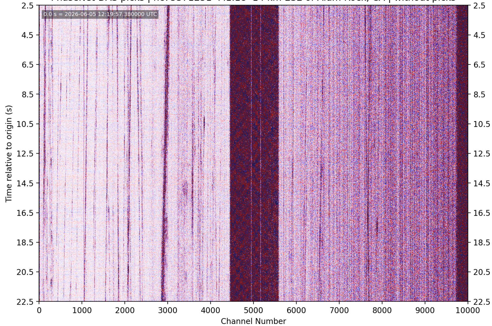
PhaseNet-DAS picks | nc75371251 M1.18 14 km ESE of Alum Rock, CA | without picks
