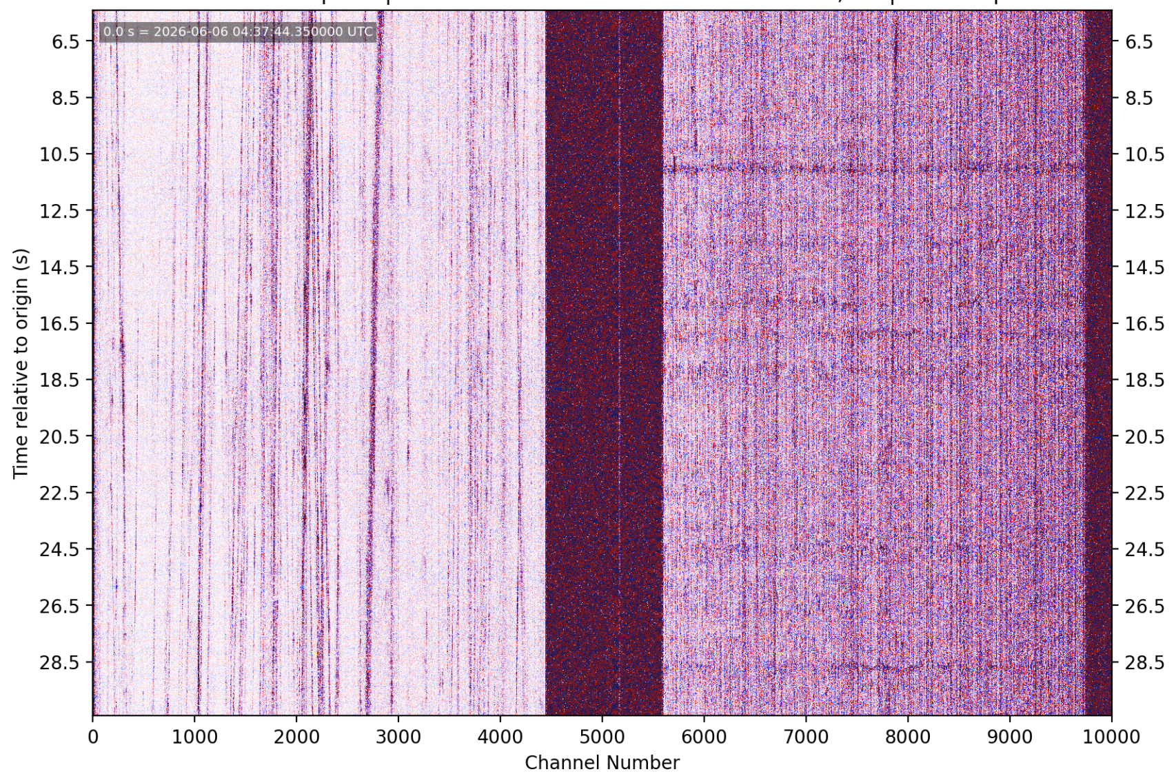
PhaseNet-DAS picks | nc75371716 M1.82 6 km E of Fremont, CA | without picks
