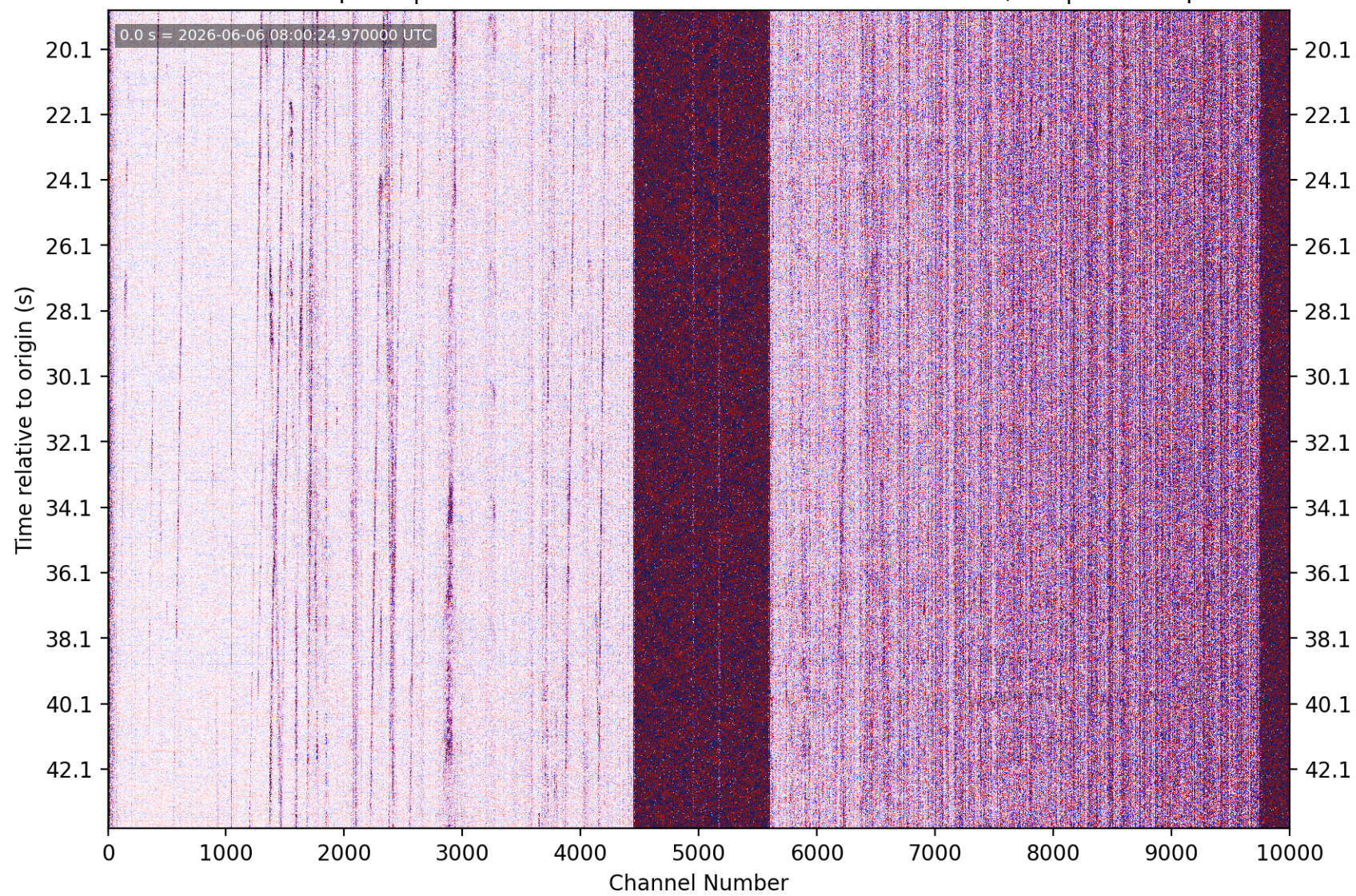
PhaseNet-DAS picks | nc75371761 M1.17 7 km ENE of San Martin, CA | without picks
