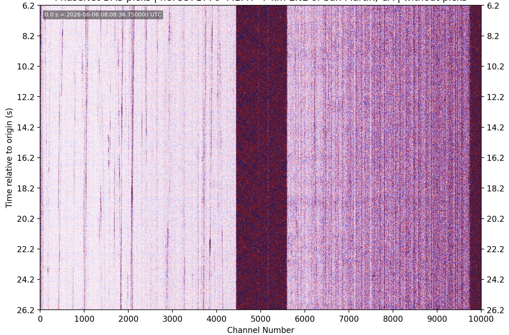
PhaseNet-DAS picks | nc75371776 M1.47 7 km ENE of San Martin, CA | without picks
