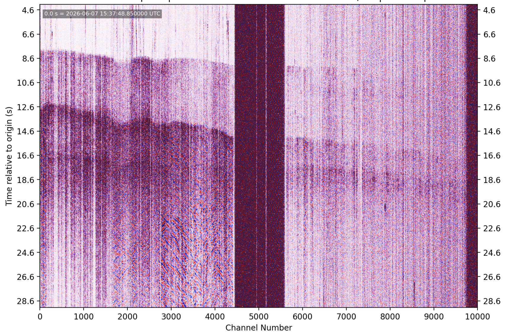
PhaseNet-DAS picks | nc75372426 M3.6 3 km SW of Alamo, CA | without picks
