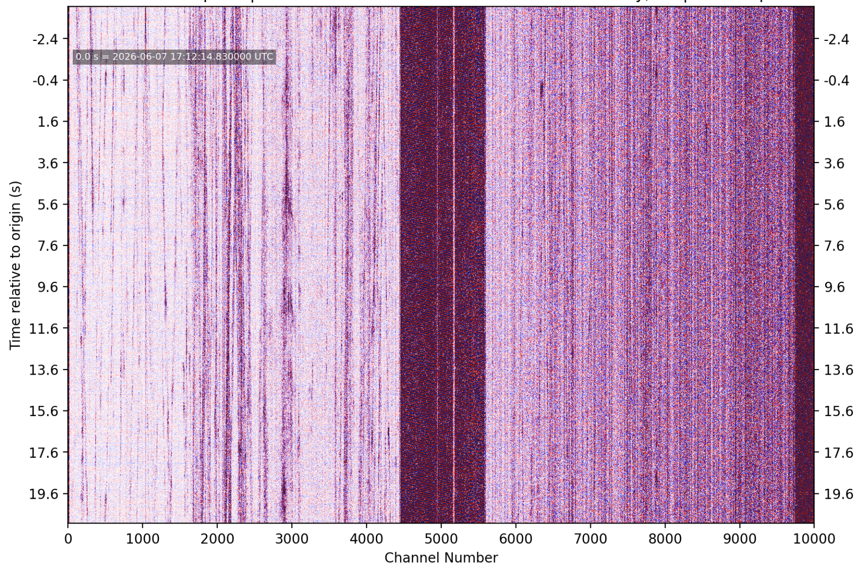
PhaseNet-DAS picks | nc75372506 M0.55 8 km SSE of Portola Valley, CA | without picks
