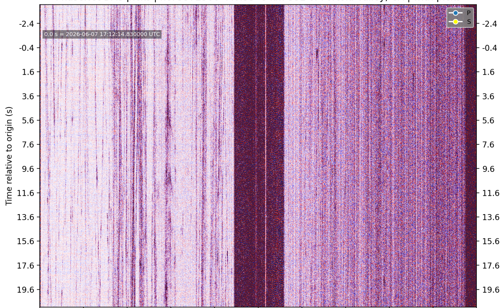
PhaseNet-DAS picks | nc75372506 M0.55 8 km SSE of Portola Valley, CA | without picks
