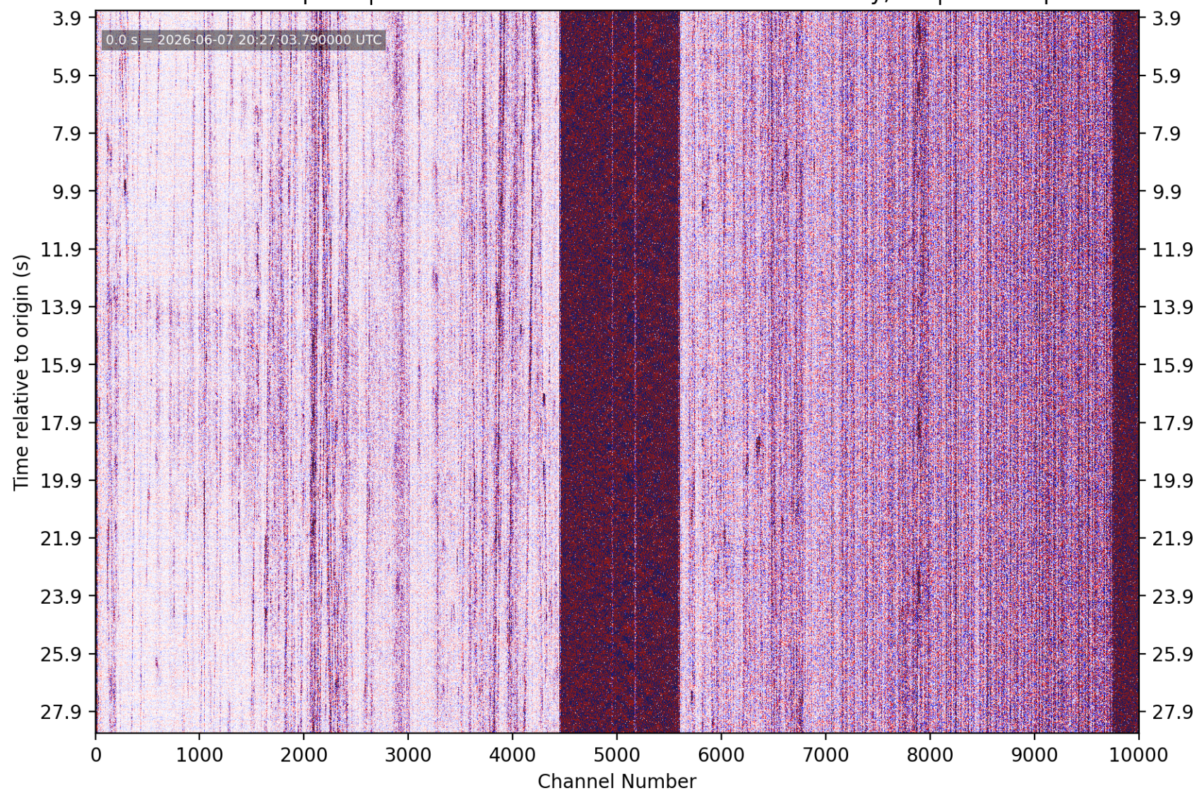
PhaseNet-DAS picks | nc75372601 M2.07 4 km ESE of Union City, CA | without picks
