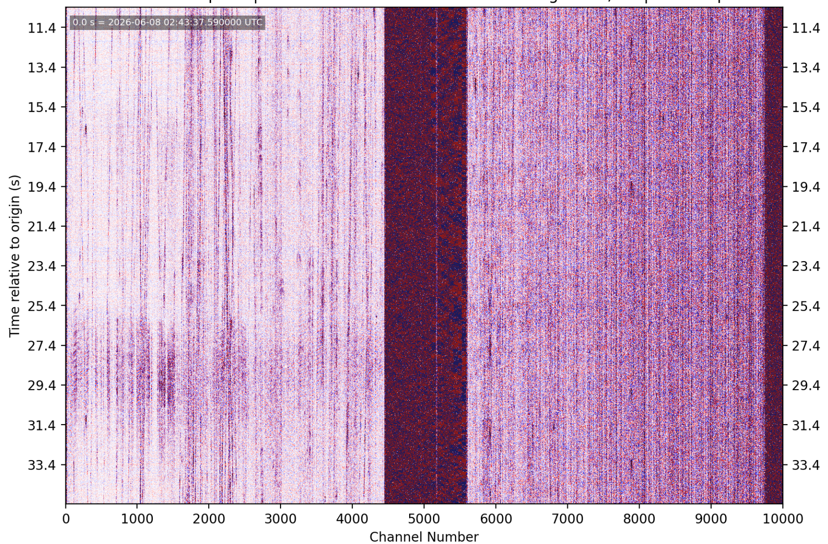
PhaseNet-DAS picks | nc75372721 M2.33 16 km N of Morgan Hill, CA | without picks
