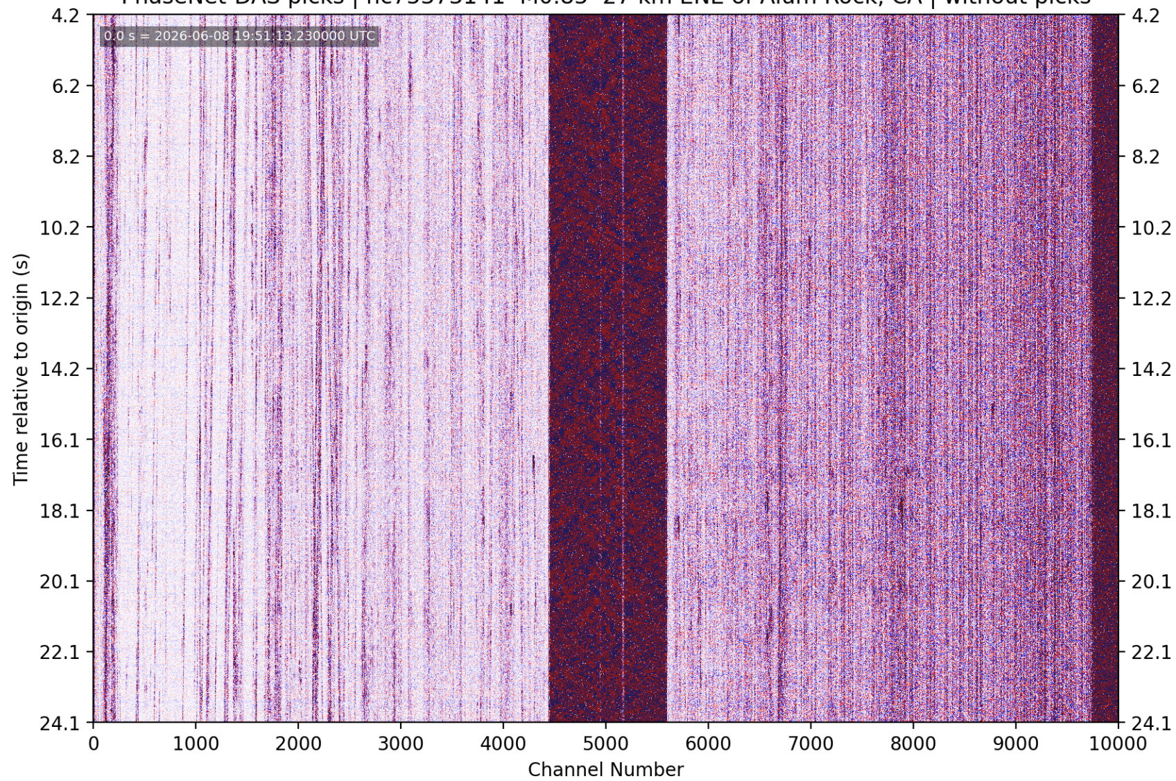
PhaseNet-DAS picks | nc75373141 M0.85 27 km ENE of Alum Rock, CA | without picks
