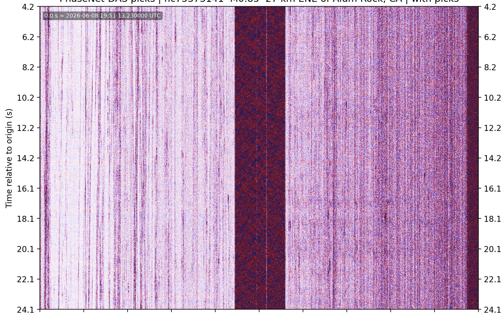
PhaseNet-DAS picks | nc75373141 M0.85 27 km ENE of Alum Rock, CA | without picks
