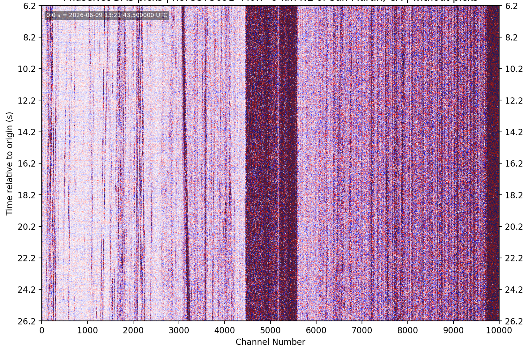
PhaseNet-DAS picks | nc75373691 M0.7 9 km NE of San Martin, CA | without picks
