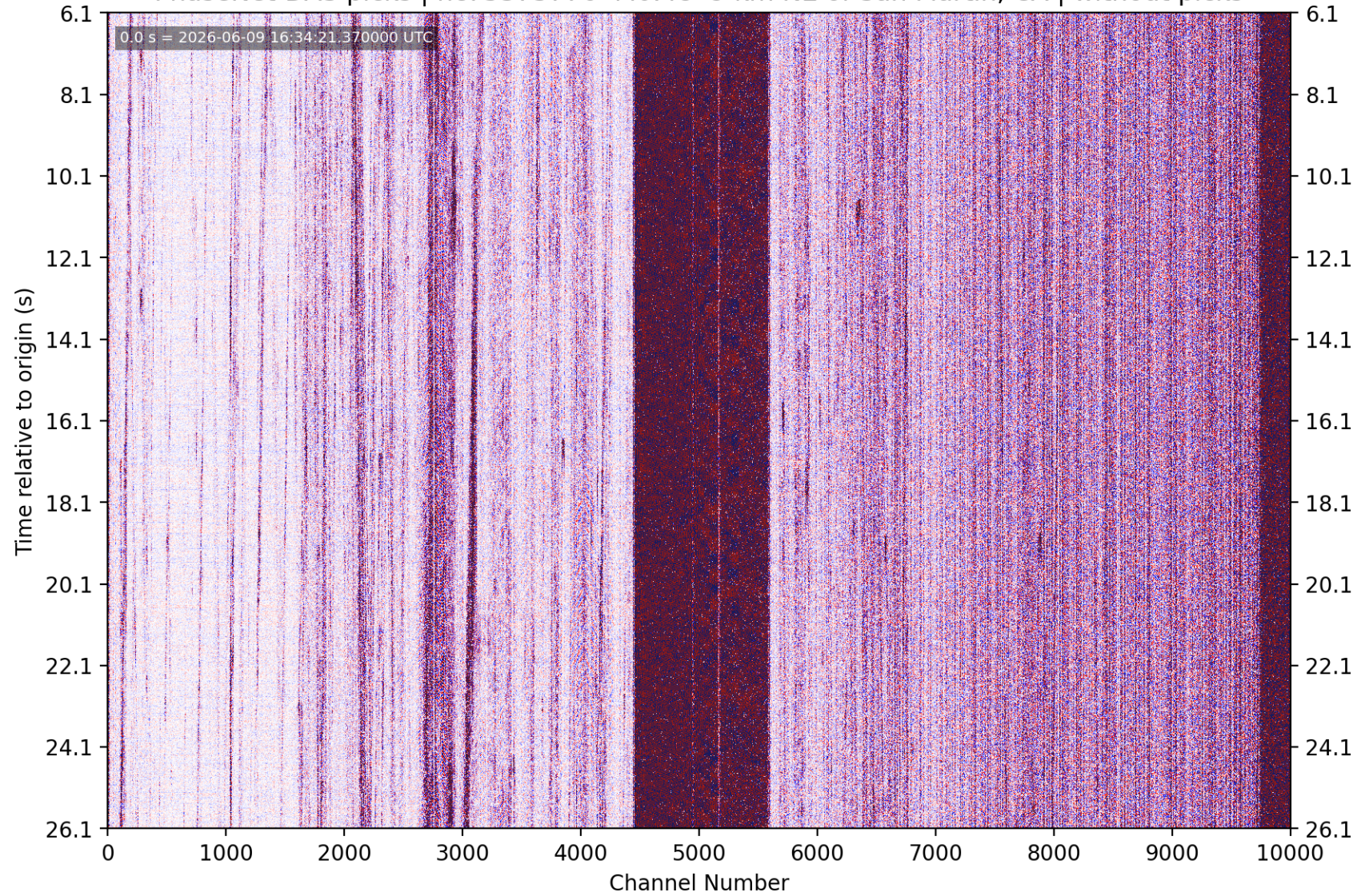
PhaseNet-DAS picks | nc75373776 M0.48 9 km NE of San Martin, CA | without picks
