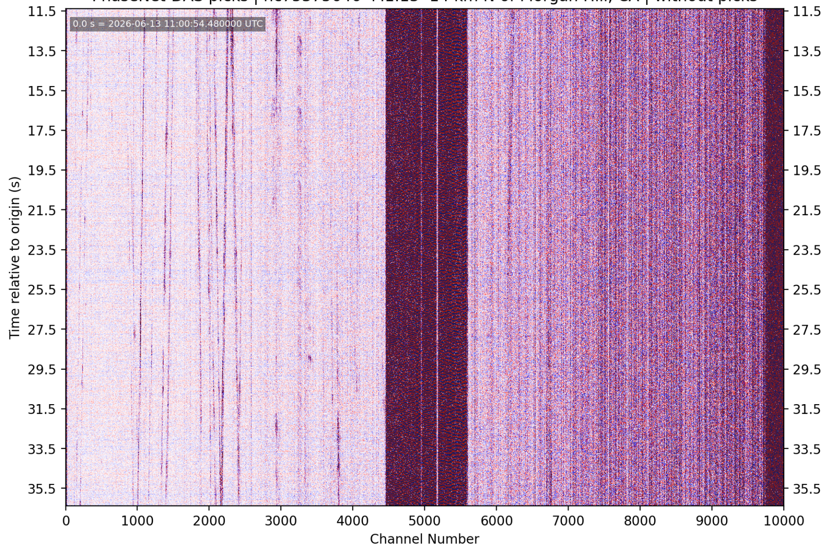
PhaseNet-DAS picks | nc75375646 M1.13 14 km N of Morgan Hill, CA | without picks
