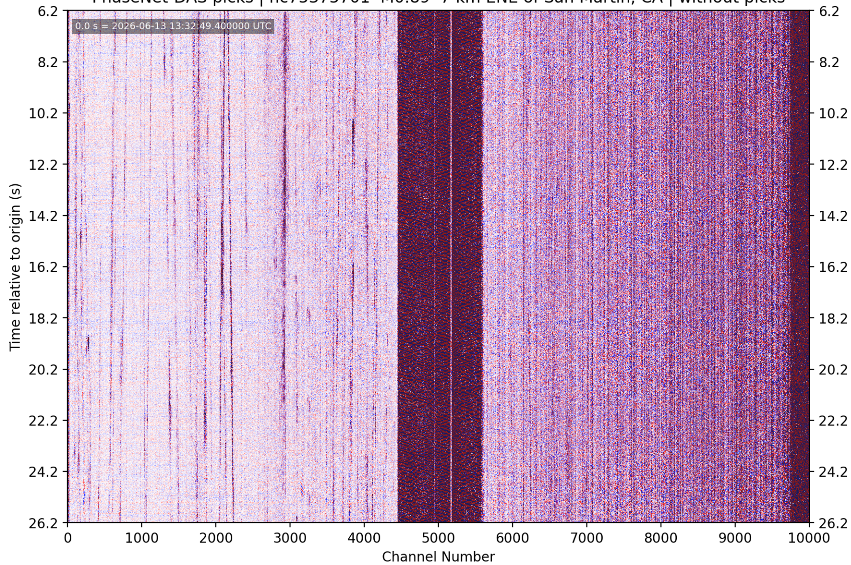
PhaseNet-DAS picks | nc75375701 M0.89 7 km ENE of San Martin, CA | without picks
