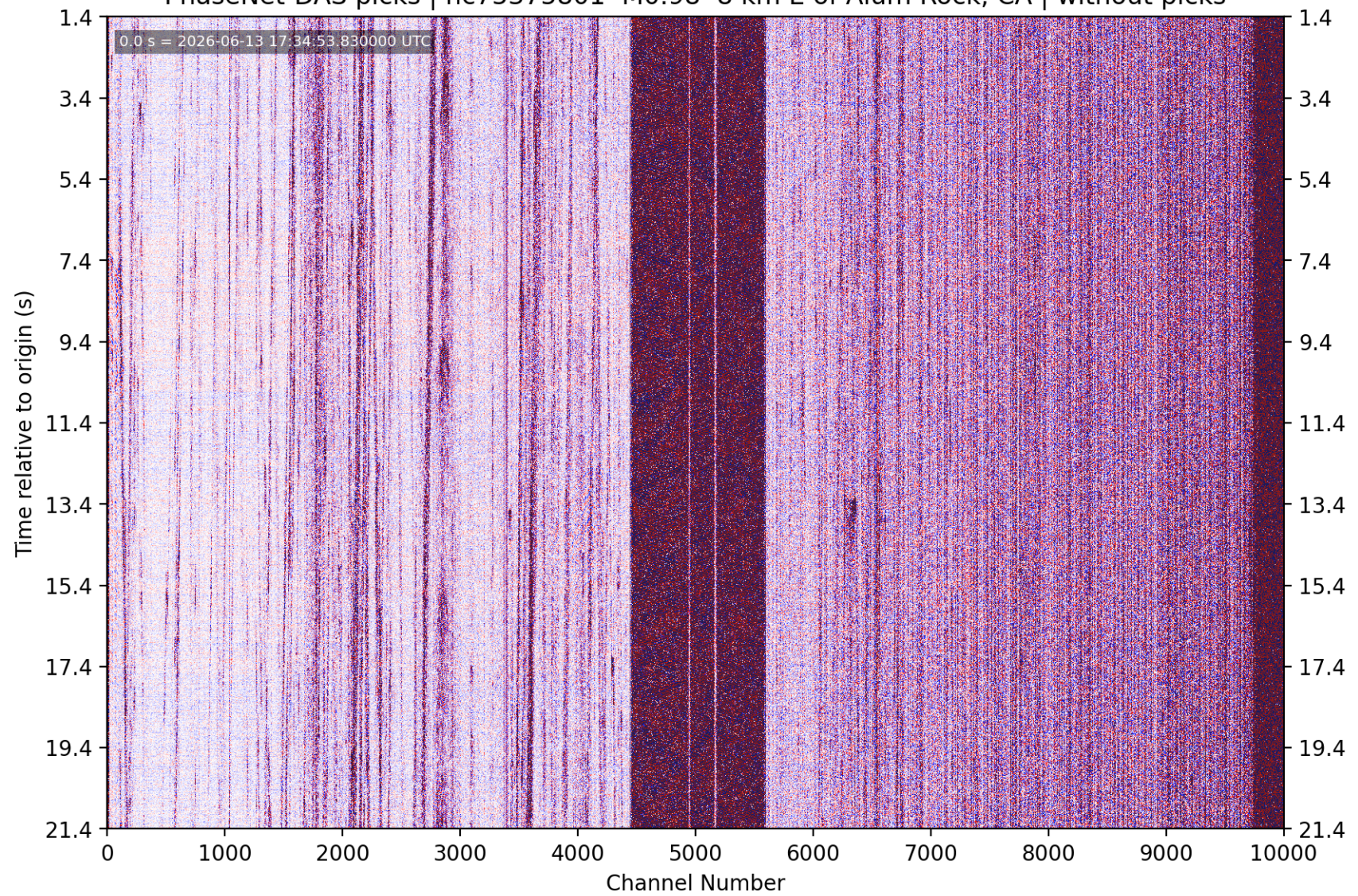
PhaseNet-DAS picks | nc75375801 M0.98 8 km E of Alum Rock, CA | without picks
